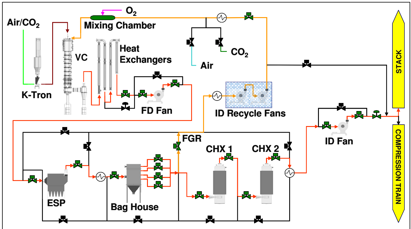
Schematic of CETC-Ottawa's 0.3MW Vertical Combustor Oxy-Fuel Research Facility and Flue Gas Treatment Units
