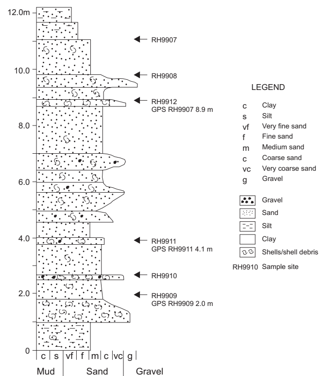
Figure 2. Stratigraphy and lithology of Haines Creek site.
