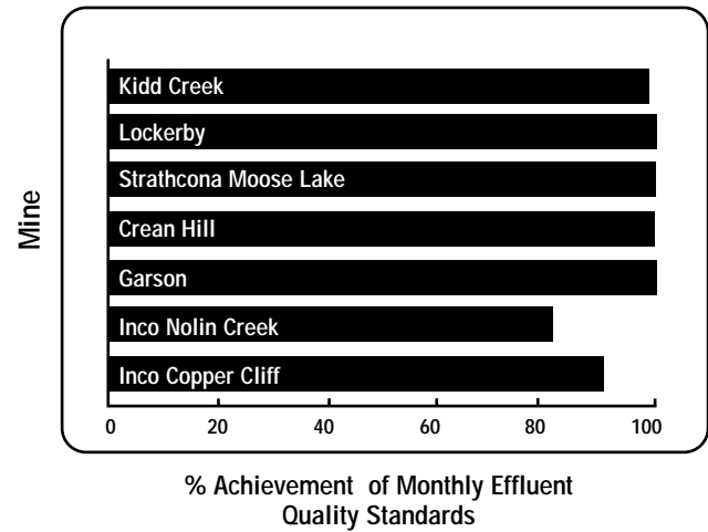
Figure 6: Performance of Mines Subject to the MMLEG in the Ontario Region in 2001
