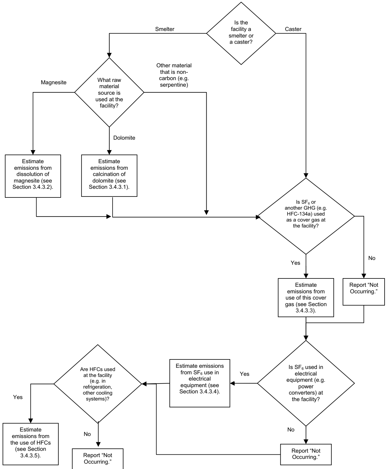
Figure 3: Decision Tree for Selecting the Method(s) for Estimating GHG Emissions from Process-related Sources
