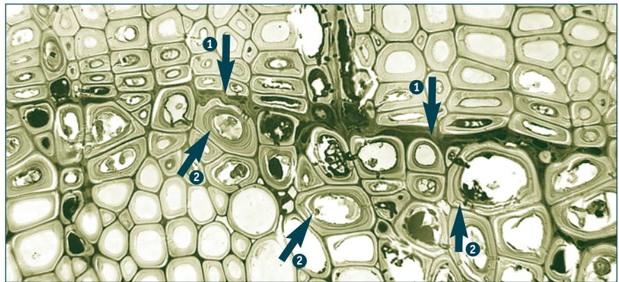
Beginning of the growth ring: collapsed cells (arrows 1) adjacent to hypertrophied cells (arrows 2). The cambium is at the bottom. Photo: D. Rioux
