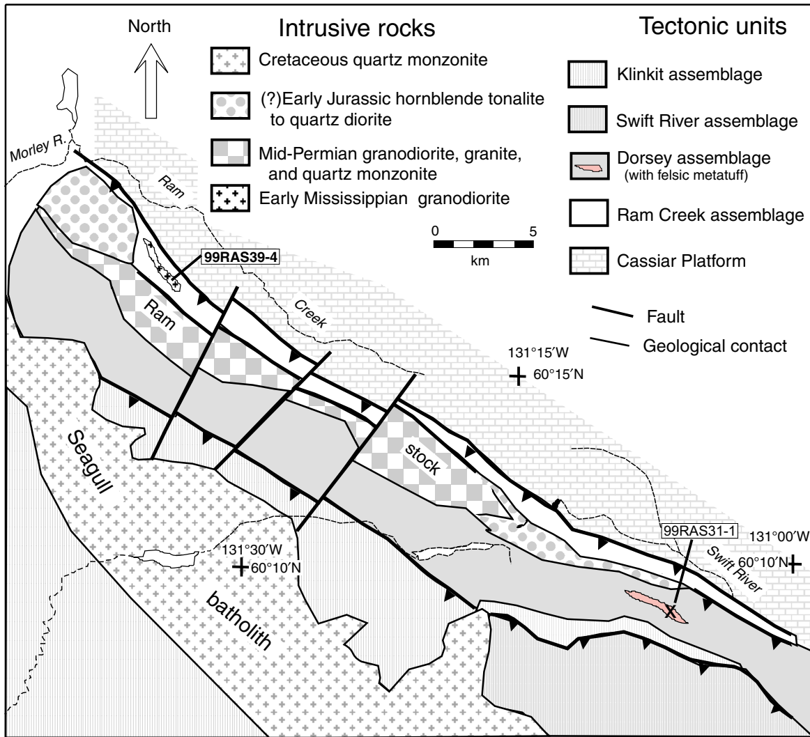
Figure 2. Distribution of rock units in northern Dorsey Terrane, showing sample sites (modified from Stevens, 1996).
