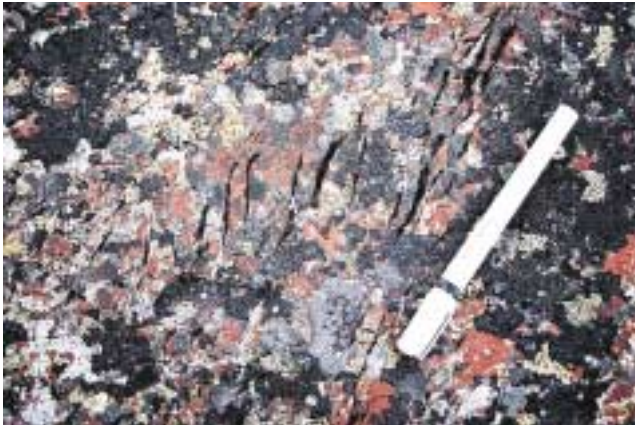
Figure 11. Tension gashes show progressive sinistral rotation, over a strain gradient leftward of the pen, from fractures trending approximately 040^\circ . The pen is oriented at 048^\circ . These are interpreted to be related to a regional set of sinistral strike-slip faults that trend about 040^\circ .
