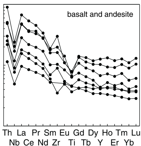
Figure 10. Primitive-mantle-normalized trace-element profiles of volcanic rocks of the Confederation assemblage (data from this study). a) McNeely sequence; b) Heyson sequence; c) Graves sequence.
