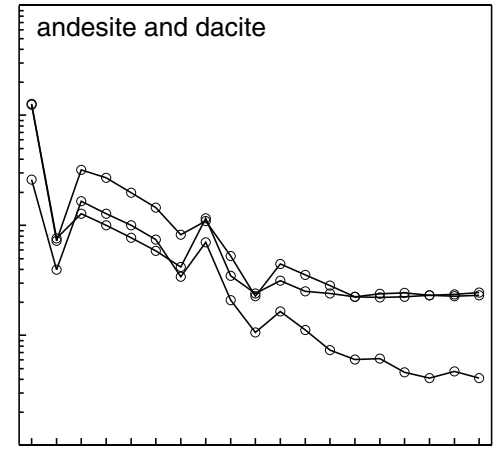
c) Graves sequence 2734–2731 Ma
