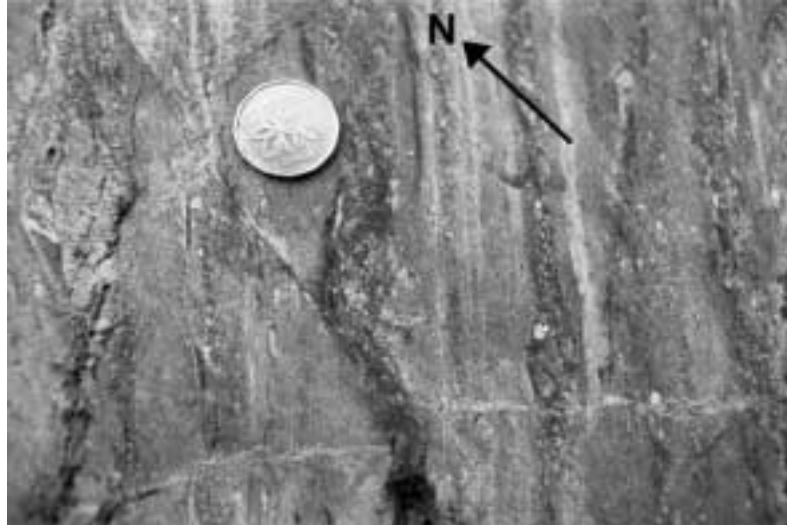
Figure 7. Interbedded sandstone and locally derived polymictic conglomerate of the Pickle Crow assemblage, showing normal grading to the northwest.
