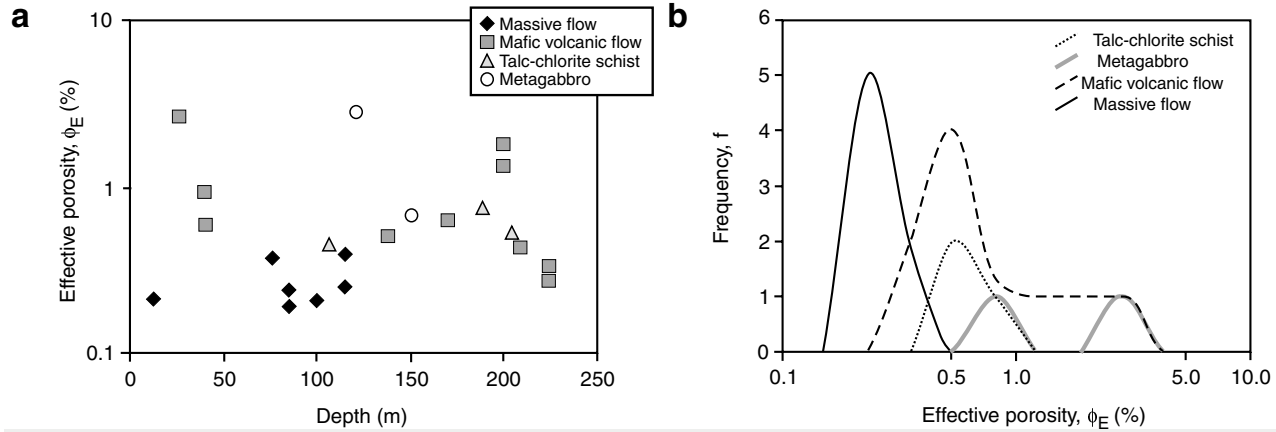
Figure 1. Effective porosity ( \phi_E ) for the mineralized and nonmineralized samples; \phi_E displayed a) as a function of depth and b) as a histogram.
