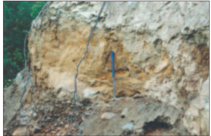
Figure 40. Measured section MIC9710 near Minto Creek, where a Diversion Creek paleosol is preserved on a Reid glaciofluvial terrace. This yellow-brown paleosol was subsequently buried by a McConnell age periglacial debris flow and protected from further erosion.
