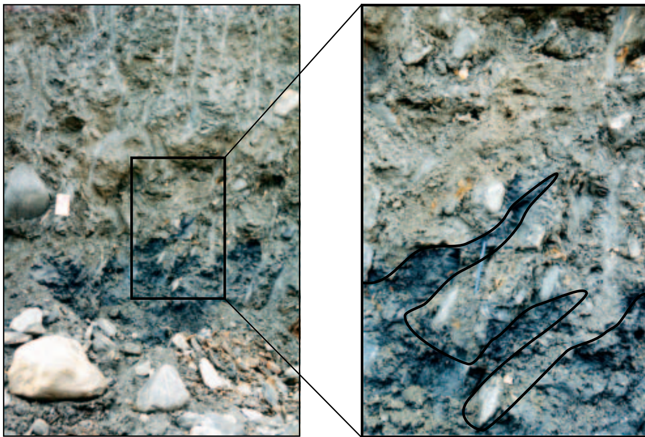
Figure 11. Facies 1 - Dmm, massive boulder cobble diamict, occurs throughout the study area, commonly in contact with bedrock. The above photos from measured section UD9703 on Upper Duncan Creek illustrate the massive, compact and disorganized nature of this facies. Bedrock slivers intrude the unit at the basal contact. This example is interpreted to be either a lodgement till or resedimented lodgement till of Reid age. Field notebook in left photo is 18 cm long.
