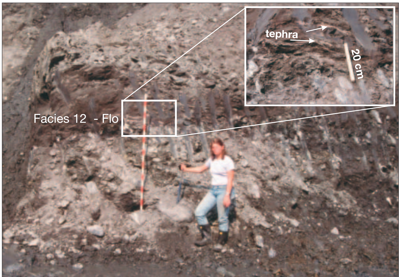
Figure 22. Facies 12 - Flo, massive to laminated organic rich silt, consists of very fine sandy silt or silt with a very high content of macerated organics and woody organic debris. Local clasts from boulder to pebble size occur in addition to accessories such as macro-organics and volcanic ash (e.g., measured section FT98-1-2, pictured here). In interglacial and Holocene settings, woody material can often be radiocarbon dated. A wood sample from this unit was ^{14}\text{C} (AMS) dated at >50 030 years B.P.
