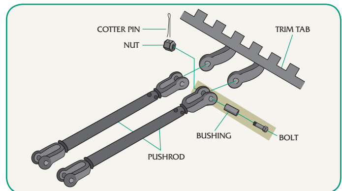
Figure 1: Artist's impression of original technical diagram
