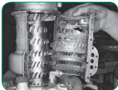
Compressor case half removed exposing damage to blades and vanes leading and trailing edges
