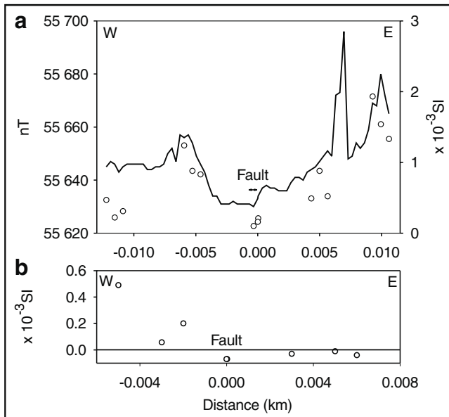
Figure 2. a) Magnetic traverse (solid line) across the northwest-trending dip-slip fault exposed at Welbury Bay, Saltspring Island (1, Fig. 1). Magnetic susceptibility values are plotted with open circles. b) Magnetic susceptibility measurements across the same structure where it is exposed on the north shore of Long Harbour.
