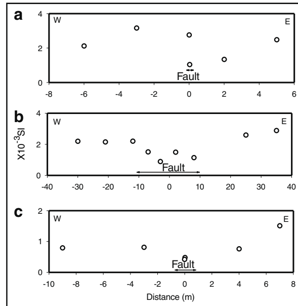
Figure 3. Averaged magnetic susceptibility values across two northeast-trending dip-slip structures on Saltspring Island. The westernmost of the two structures (2, Fig. 1) comprises at least two distinct strands, one of which is approximately 30 to 40 cm wide (a) and the other, 10 to 20 m wide (b). The eastern structure (3, Fig. 1) consists of a single fault strand approximately 0.5 m wide (c).
