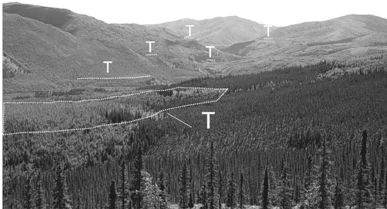
Figure 4. View up Grand Valley (also called 'South Rosebud') Creek from UTM 7V E634986, N7010873 at approximately 790 m elevation and 335 m above the floor of Grand Valley Creek. Areas marked by 'T' are glaciofluvial.
