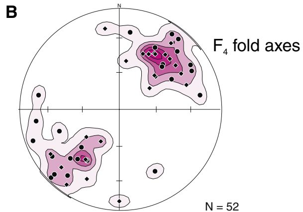
Figure 5. Stereonet plot of poles to S_4 fabric ( A ) and measured F_4 axes ( B ). For both plots, circles represent data from the North Portage deposit and diamonds from the Third Portage deposit. C ) Photograph of F_4 folds from the North Portage area.
