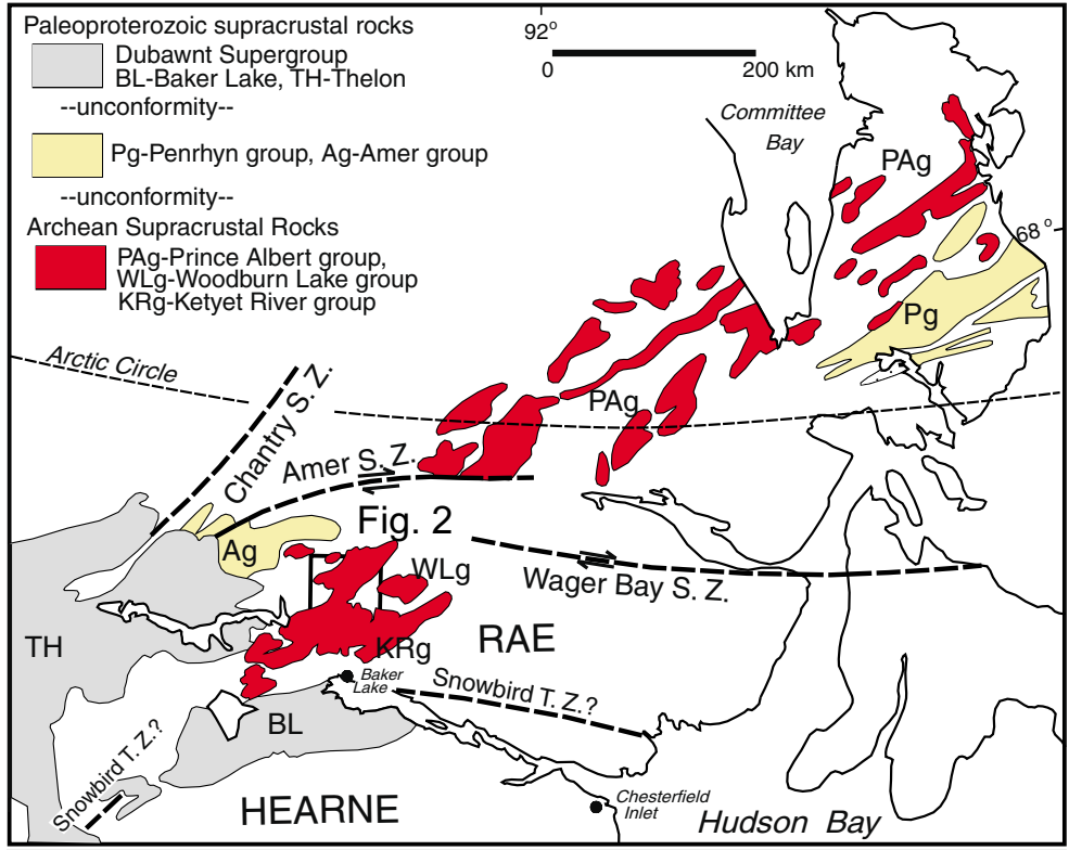
Figure 1. Regional geological sketch map of the western Churchill Province, showing the distribution of Archean supracrustal rocks in the Woodburn Lake group (WLg), the Prince Albert group (PAg), and the Ketyet River group (KRG) relative to the Paleoproterozoic suites of the region (Zaleski et al., 1997b).
