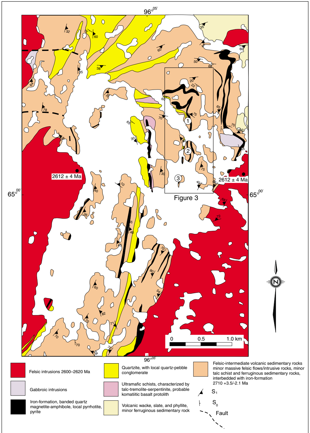
Figure 2. Simplified geological map of the Woodburn Lake group in the Meadowbank area (Zaleski et al., 1997a, 1999a). Circled numbers: 1. North Portage deposit, 2. Third Portage deposit, 3. Goose Island deposit. The Bay Zone deposit is immediately southwest of Third Portage.
