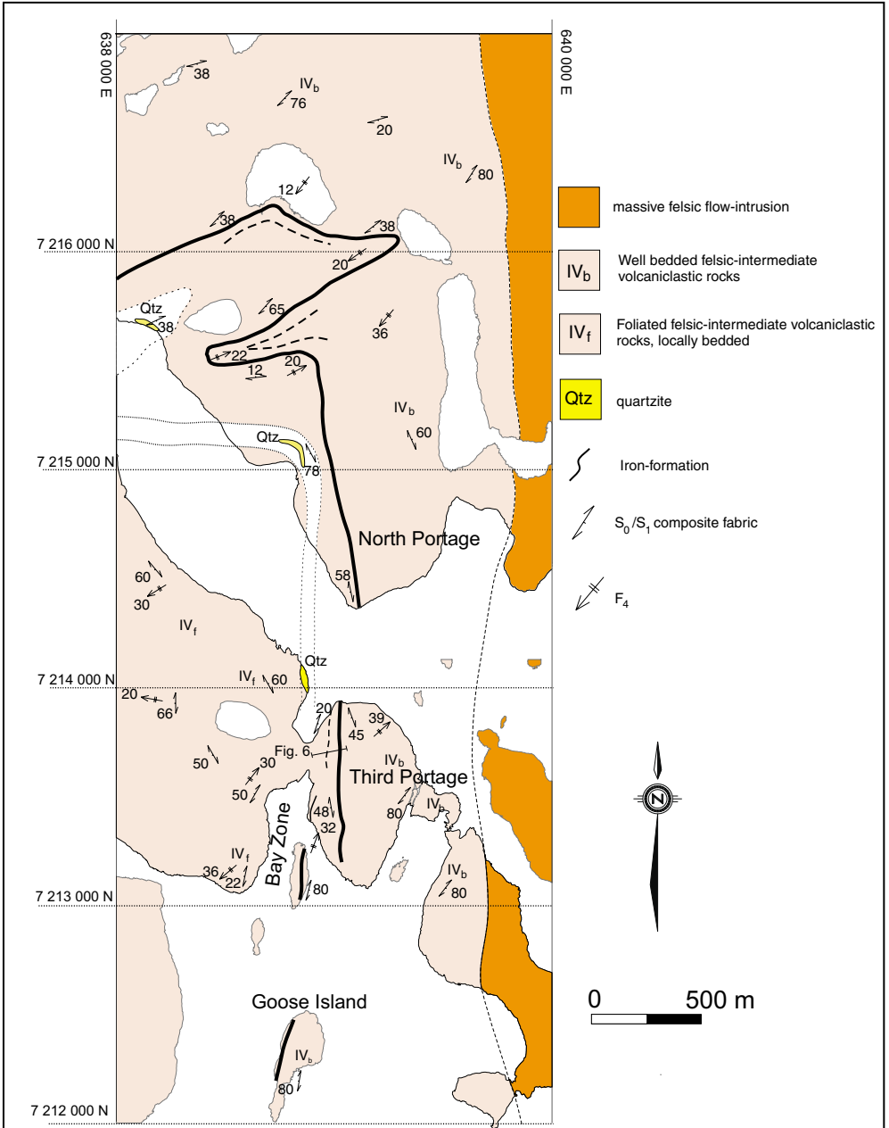
Figure 3. Simplified geological map of the Meadowbank deposits showing the distribution of the rock types and tectonic fabrics. Cross-section in Figure 6 is shown in the Third Portage deposit.
