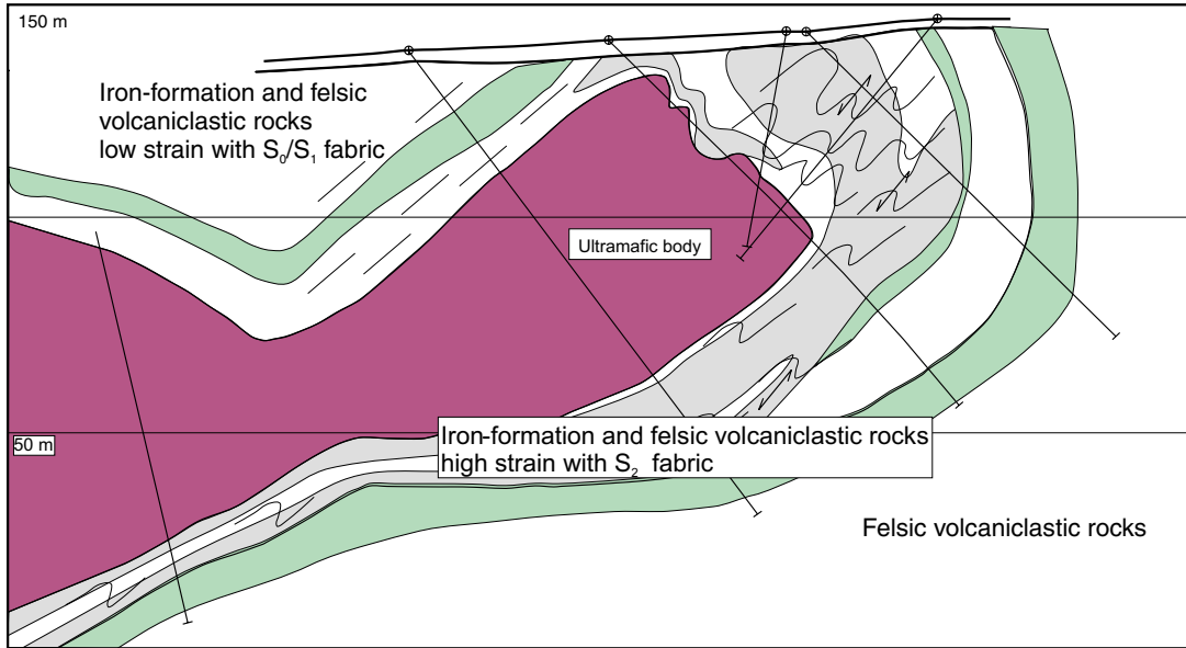
Figure 6. Simplified cross-section through the Third Portage deposit at section 1+80N. This shows the distribution of gold and deformation fabrics around the ultramafic body. The shaded area represents an interpreted mineralized envelope; any material within the shaded areas will average greater than 1.0 g/t gold.
