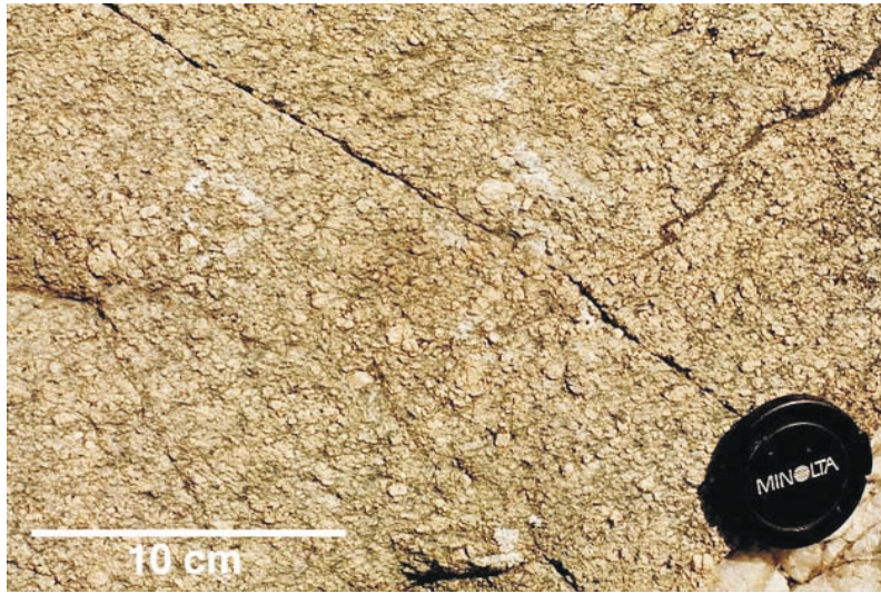
Figure 9. Arkosic grit forming the basal layer of the North Wanipigow assemblage, Wanipigow Lake.
