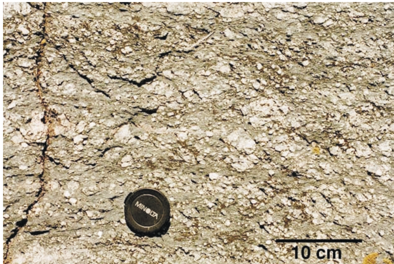
Figure 7. Basal conglomeratic grit containing angular tonalite clasts in a chloritic matrix.
