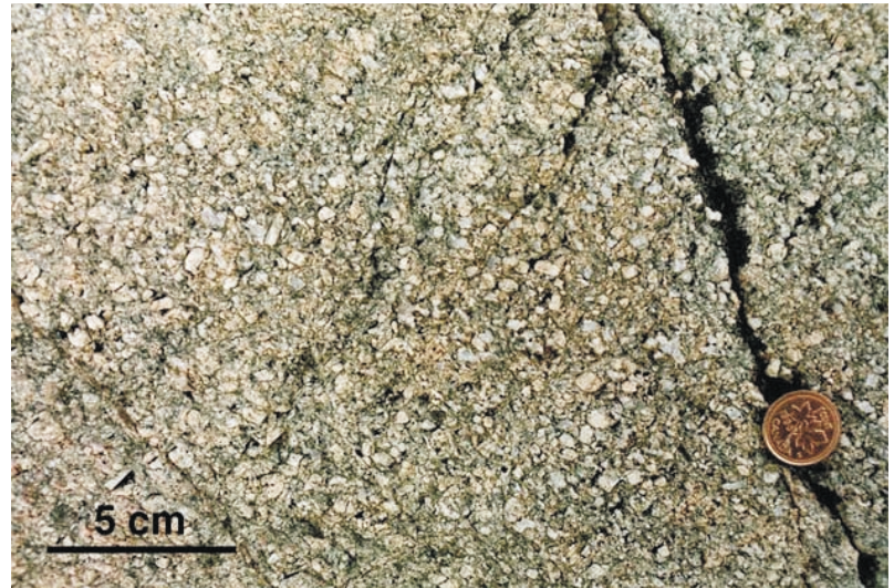
Figure 6. Arkosic grit of the Lewis-Storey assemblage showing angular quartz and plagioclase granules.
