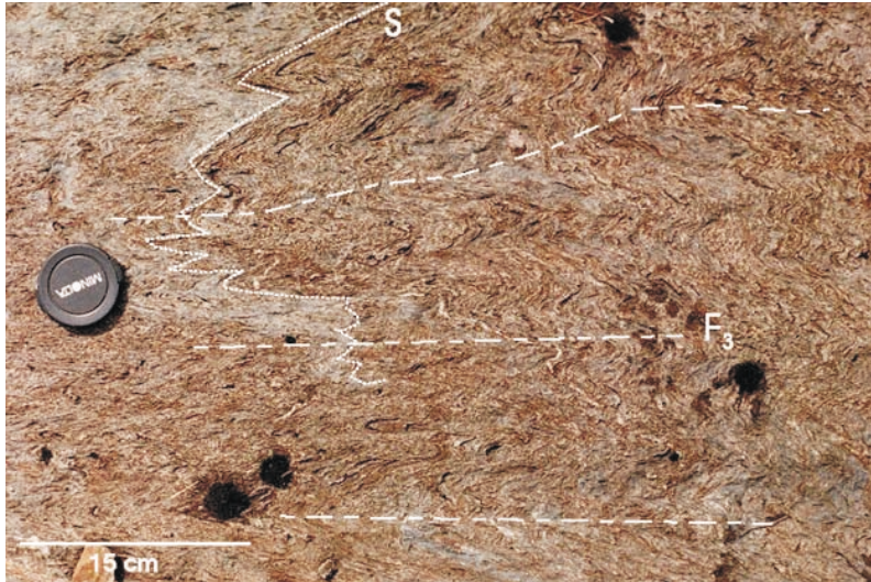
Figure 17. Overprinting relationship in the Seymourville shear zone: F_3 folds overprint an early fabric ( S ), which may be S_1 or composite S_1 – S_2 in chlorite-carbonate-quartz schist.
