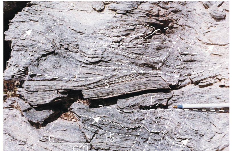
Figure 10. Stretched-pebble conglomerate (flattened clasts indicated by arrows) of the Hole River sequence, showing a strong S_1 tectonic lamination, tight F_1 Z-fold, and open F_2 crenulations.
