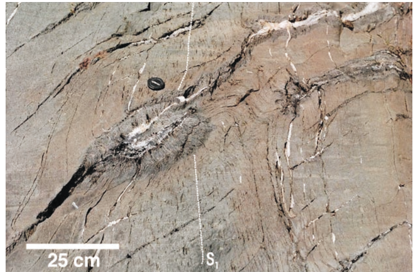
Figure 14. Tourmaline-quartz-carbonate vein cutting S_1 -foliated mafic sill, Lewis-Storey assemblage. Note tourmaline replacement along S_1 planes.
