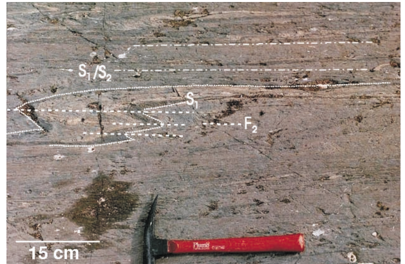
Figure 16. D_2 shear zone developed through fold-limb transposition from highly D_1 -strained basalt of the Black Island assemblage.
