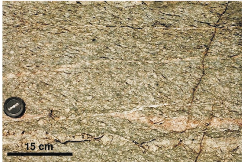
Figure 3. Dextral D_1 shear bands developed in tonalite, East Shore Plutonic Complex.
