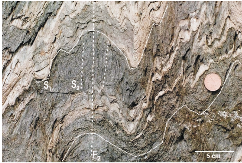
Figure 15. F_2 folds and associated axial plane S_2 cleavage affecting strong S_1 fabric. The dark and light layers can be traced into pillow cores and selvages respectively, in weakly foliated pillow basalt.
