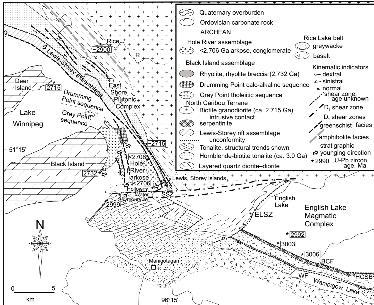
Figure 2. Tectonic map of the eastern Lake Winnipeg–Wanipigow Lake area (modified from Ermanovics, 1981; Weber, 1991). Many small islands in eastern Lake Winnipeg are not shown at this scale. BCF = Beaver Creek Fault; ELSZ = English Lake shear zone; HCSB = Hay Creek serpentinite belt; SSZ = Seymourville shear zone; WF = Wanipigow Fault.
