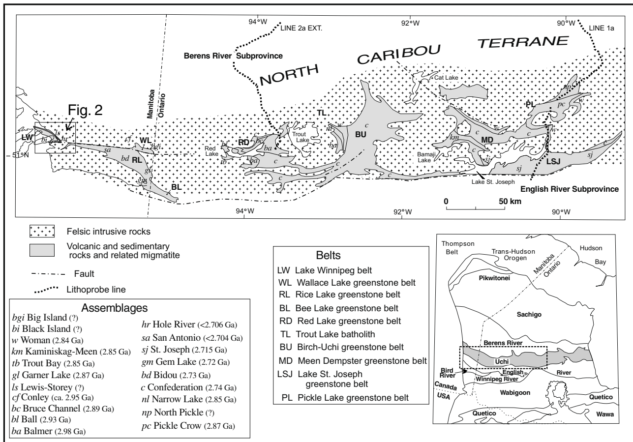
Figure 1. Tectonic map of the western Uchi Subprovince showing major greenstone belts and assemblages.
