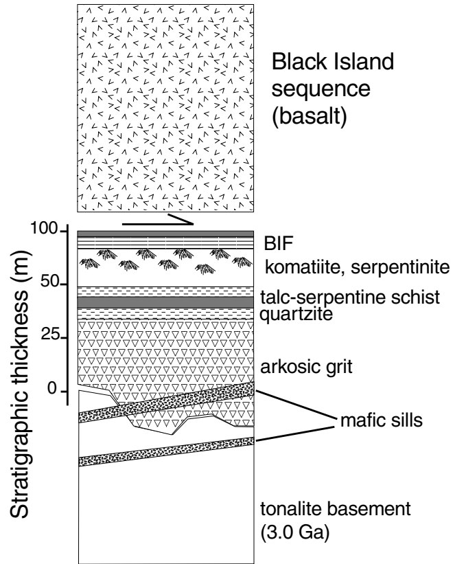
Figure 5. Composite stratigraphic column showing major units of the Lewis-Storey assemblage.
