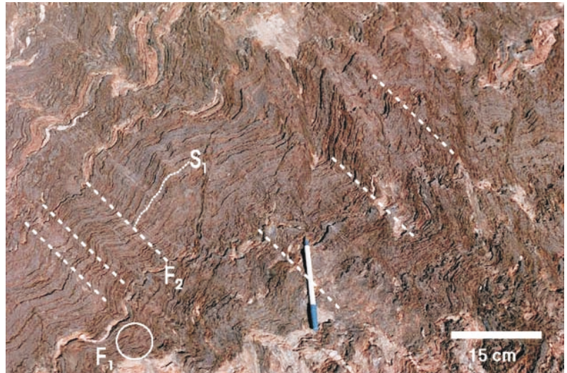
Figure 12. Chlorite-carbonate-quartz schist developed in D_1 shear zone in Black Island basalt. Note minor F_1 fold in the lower left corner and F_2 crenulations.
