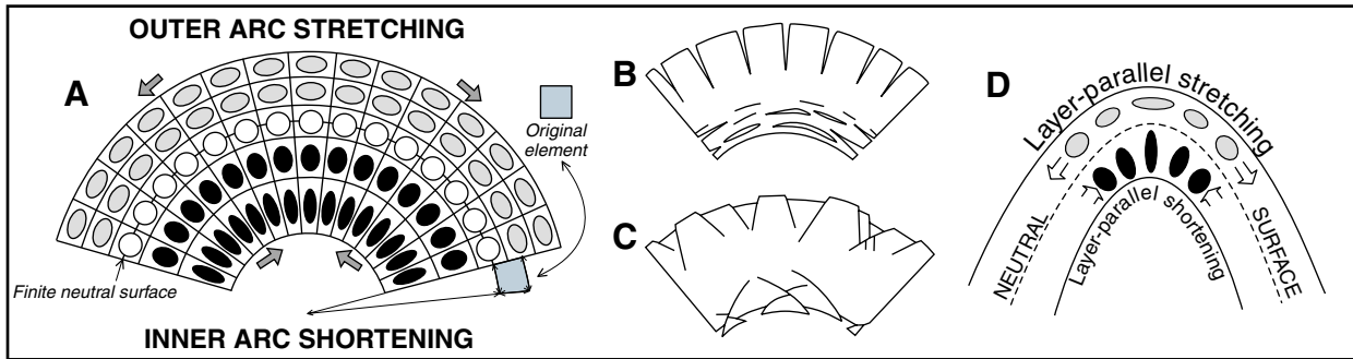
Figure 6. A) Geometrical features of fold formed under conditions of tangential longitudinal strain in a competent layer. B) Extension fissures. C) Conjugate shear faults ( after Ramsay and Huber, 1987 ). D) Fold-related layer-parallel stretching and shortening ( after Davis and Reynolds, 1996 ).
