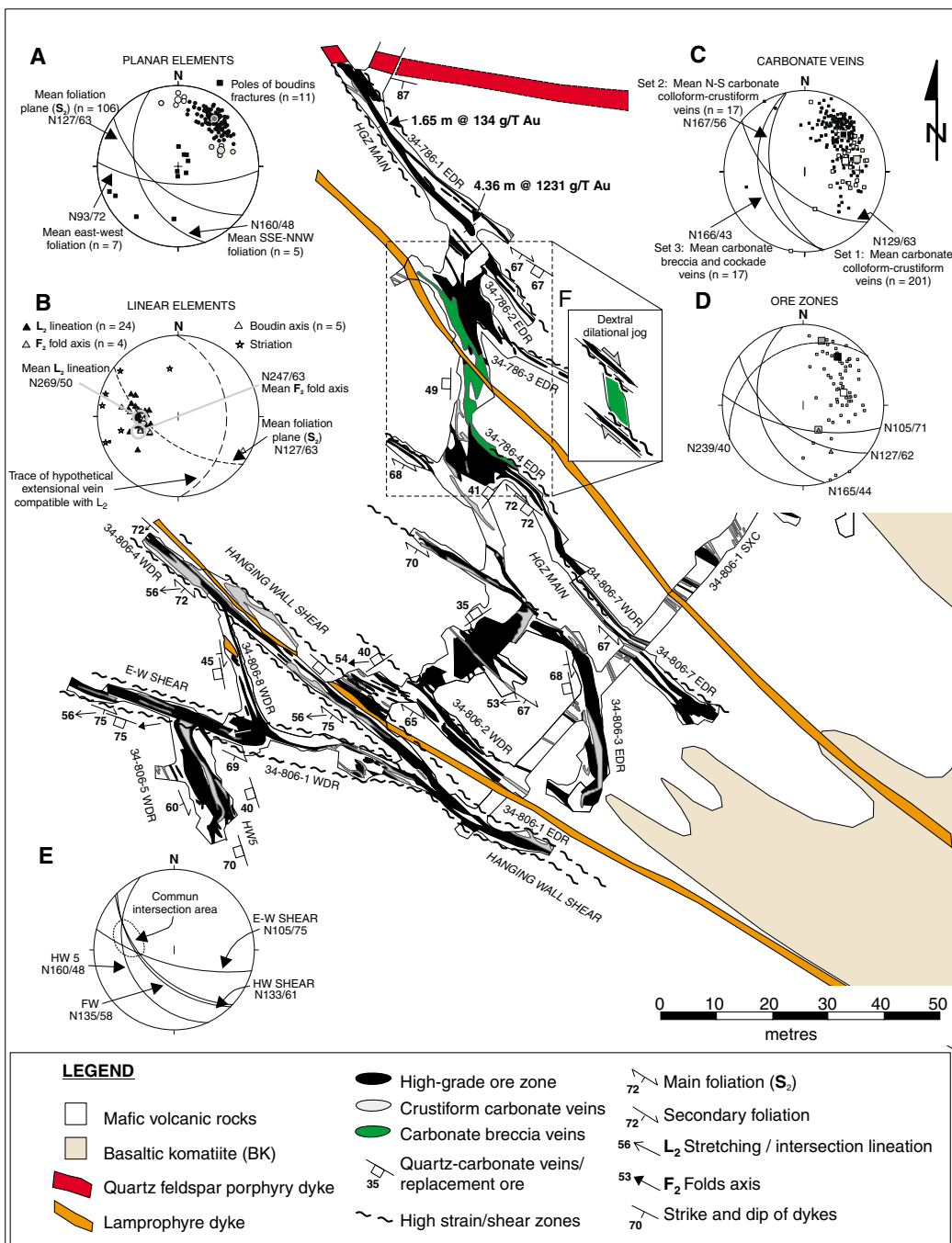
Figure 2. Detailed geology of the High Grade zone level 34 at Red Lake mine (modified from Goldcorp Inc. geological data). Stereonets are equal area projections (lower hemisphere).
