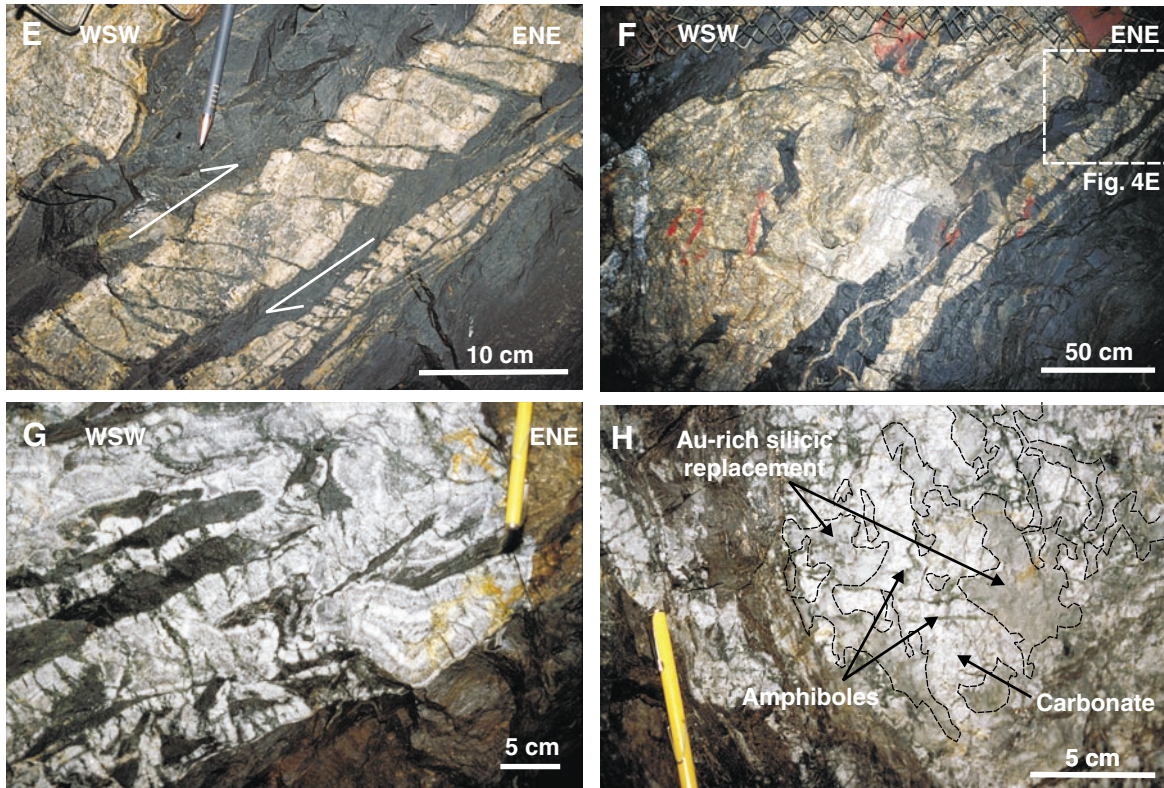
Figure 4. E) Section view of asymmetric boudins deforming colloform carbonate vein, hanging-wall-side-up. F) Section showing northwest-trending type 3 breccia vein with colloform-cockade breccia texture. G) Colloform and cockade textures in carbonate extensional breccia vein. H) Gold-rich quartz replacing carbonate vein.
