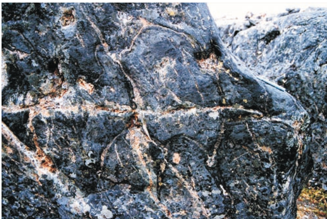
Figure 9. Small cliff section on outcrop of the Bravo Lake Formation showing well-preserved pillow structures in basalt. Located in large klippen southwest of Nadluardjuk Lake. Pillow in the centre of photograph is approximately 40 cm wide.
