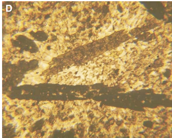
Figure 3. A) Banded amphibolite gneiss at the contact between overlying volcanic rocks and granitoid rocks in the core of the Aylmer dome; B) photomicrograph of banded amphibolite showing banding of amphibole-poor and amphibole-rich layers (40x magnification); C) pillowed mafic volcanic rock with well preserved selvages; D) photomicrograph of andesite showing coarser grained amphibole in a finer grained quartzofeldspathic groundmass (40x magnification).
