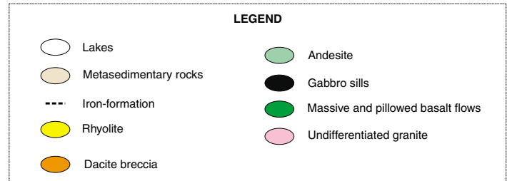
Figure 2. Simplified geological map of the Aylmer dome.
