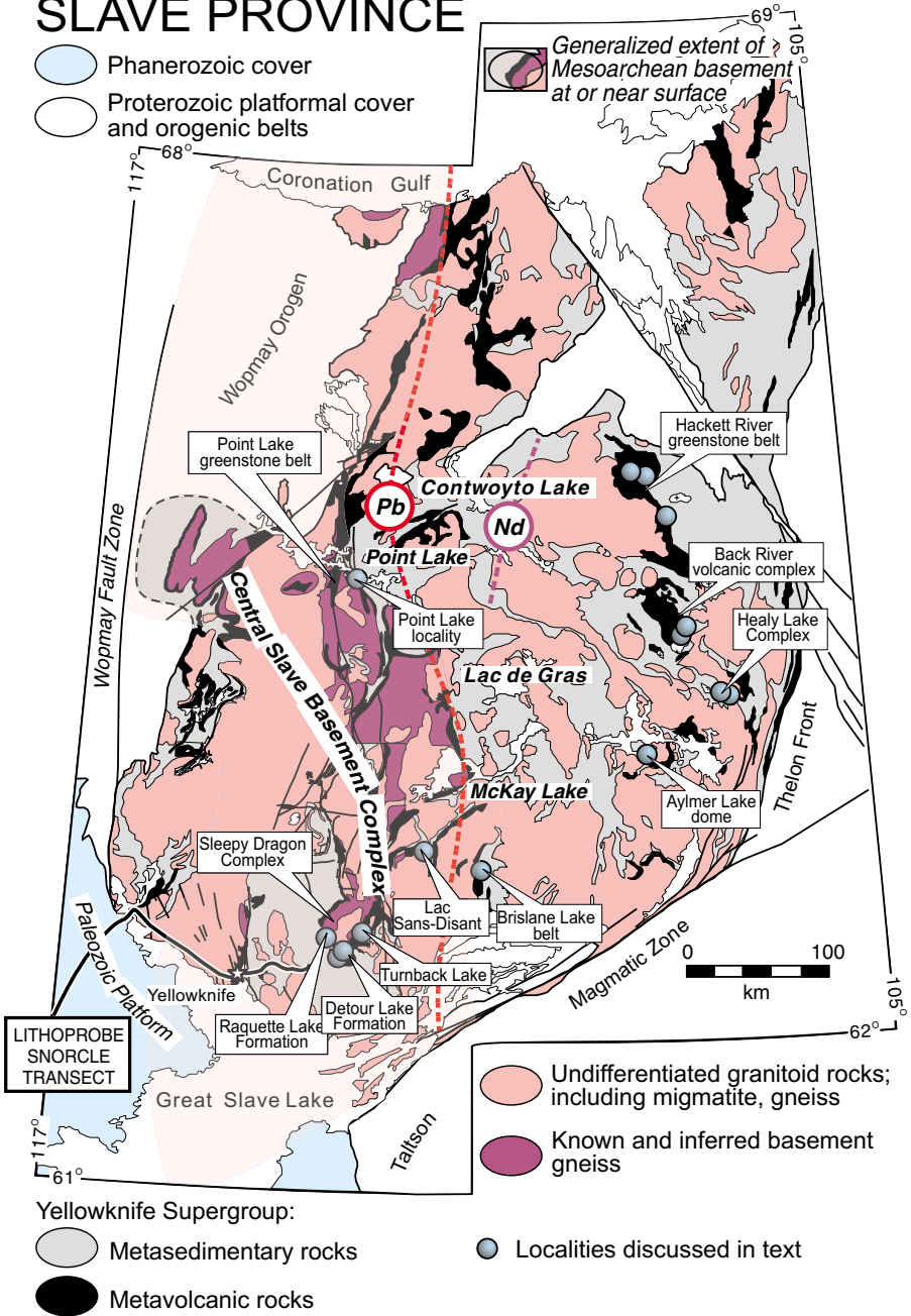
Figure 1. Geological map of the Slave Province highlighting localities discussed in the text.
