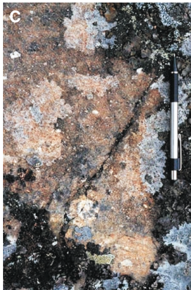
Figure 4. A) Schematic section of stratigraphic relationships in the Point Lake area, highlighting the four temporally distinct unconformities discussed in the text. Each unconformity is overlain by coarse clastic rocks. Unconformity '3' is of particular interest here and is thought to correlate with the sub-Raquette Lake unconformity 280 km to the south. B) Conglomerate with angular to rounded Augustus Granite cobbles overlying unconformity '3' (scale bar is 15 cm). C) Pebbly, greywacke-like sandstone overlying the basal conglomerate of B) (pen is 15 cm).
