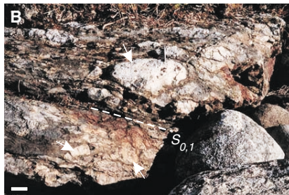
Figure 2. Stratigraphic fence diagram of the Raquette Lake and Detour Lake formations based on geological mapping of the southwestern and southern flanks of the Sleepy Dragon Complex and 27 measured sections across apparent stratigraphy. Locations of field photographs (A to D) are shown on the section (pen or scale bar is 15 cm in all photographs). A) Highly deformed polymict basal conglomerate of the Detour Lake Formation on northeast Detour Lake. B) Similar to A); note large the granodiorite boulders (at arrows). C) Thinly layered intermediate volcanoclastic rocks that make up most of the Detour Lake Formation. D) Older gneissic enclaves (at arrows) in the Ross Lake Granodiorite.
