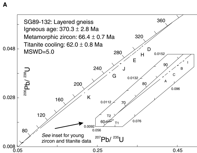
Figure 3. Uranium-lead concordia diagrams with error ellipses plotted at the 2\sigma level of uncertainty. A) Layered gneiss sample SG89-132. B) Quartzite sample SG89-98-6. Fractions A, B and C on the main diagram are plotted as crosses that do not reflect analytical uncertainty. See Table 1 for precisions and inset with ellipse for fraction A plotted at the 2\sigma level of uncertainty.
