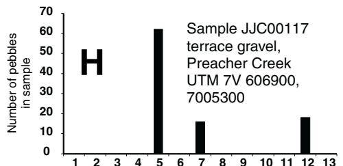
Figure 3. Counts of pebbles sampled from gravel units within glacial limits mapped by Bostock (1966; histograms B–C) and beyond them but within limits mapped by Duk-Rodkin (1999; D–H). Histogram A was determined on a sample taken from a valley-train deposit along Indian River.
