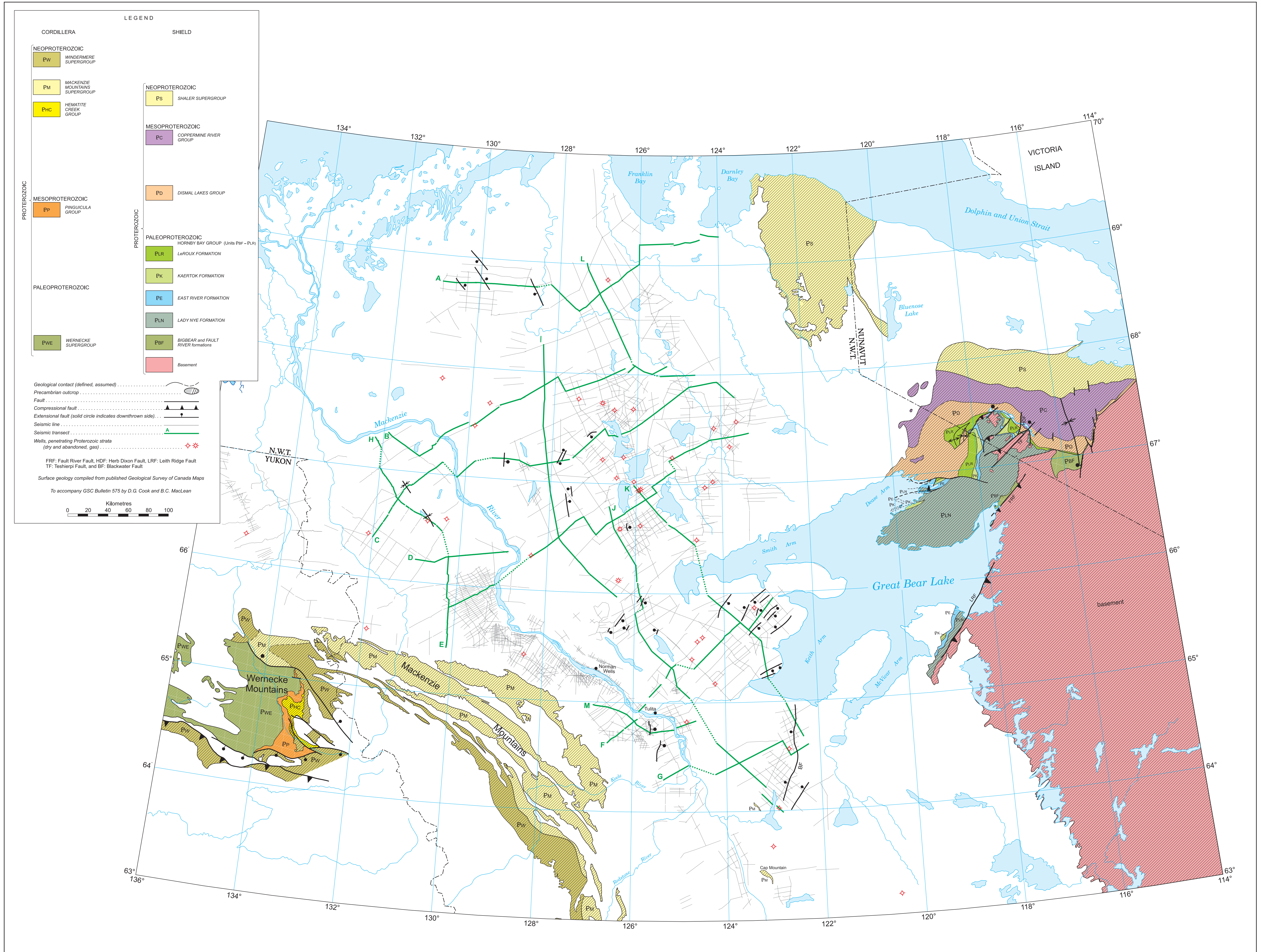
Figure 63. Map showing Phanerozoic extension features having Proterozoic antecedents.
