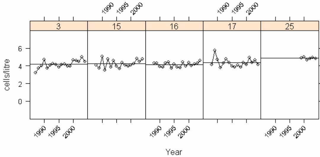
Fig. 9. Maximum density ( \text{cells}\cdot\text{L}^{-1} ) of M. rubrum at Stations 3, 15, 16, 17, and 25 on a log-transformed scale. Solid line indicates the mean of the log cell concentrations.
