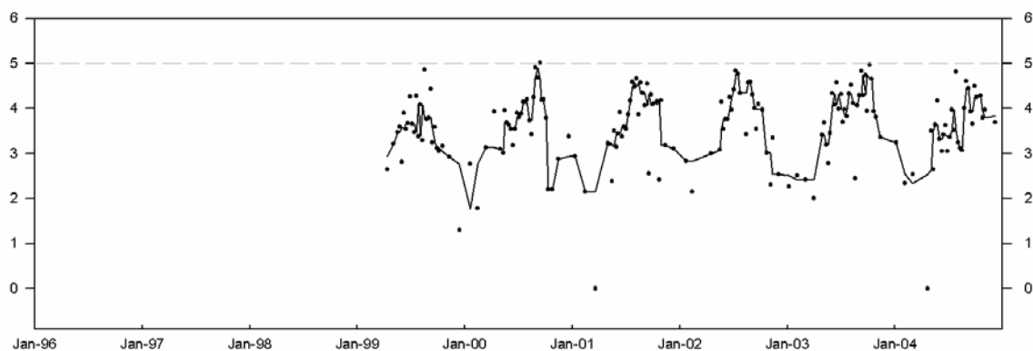
Fig. 7B. Concentrations ( \text{cells}\cdot\text{L}^{-1} ) of M. rubrum from mid-Passamaquoddy Bay (#25) on a log-transformed scale (1999-2004). Dotted line indicates the 100\,000\ \text{cells}\cdot\text{L}^{-1} concentration.
