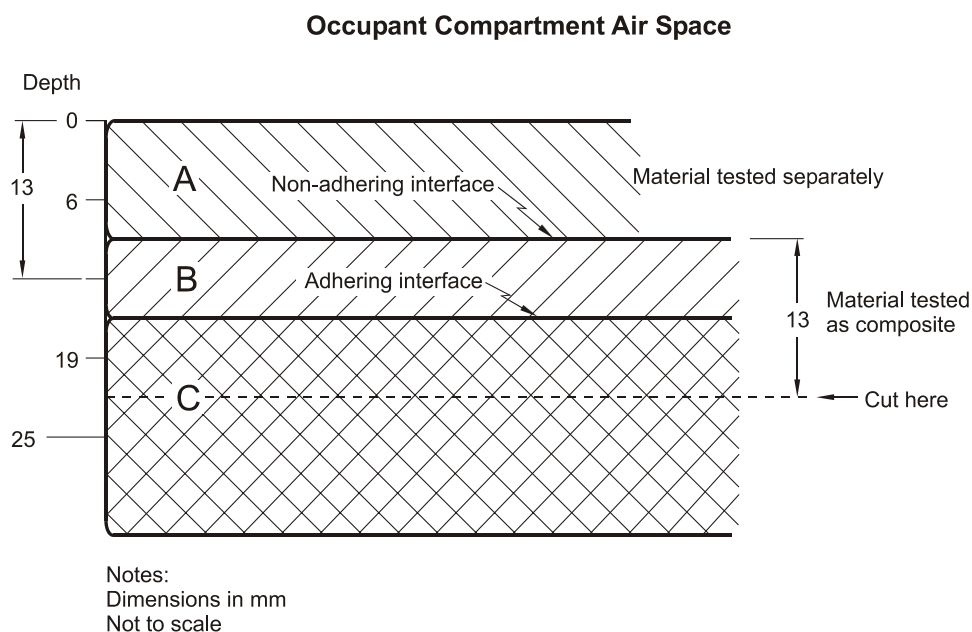
Figure 7 — Thickness of the Test Specimen
