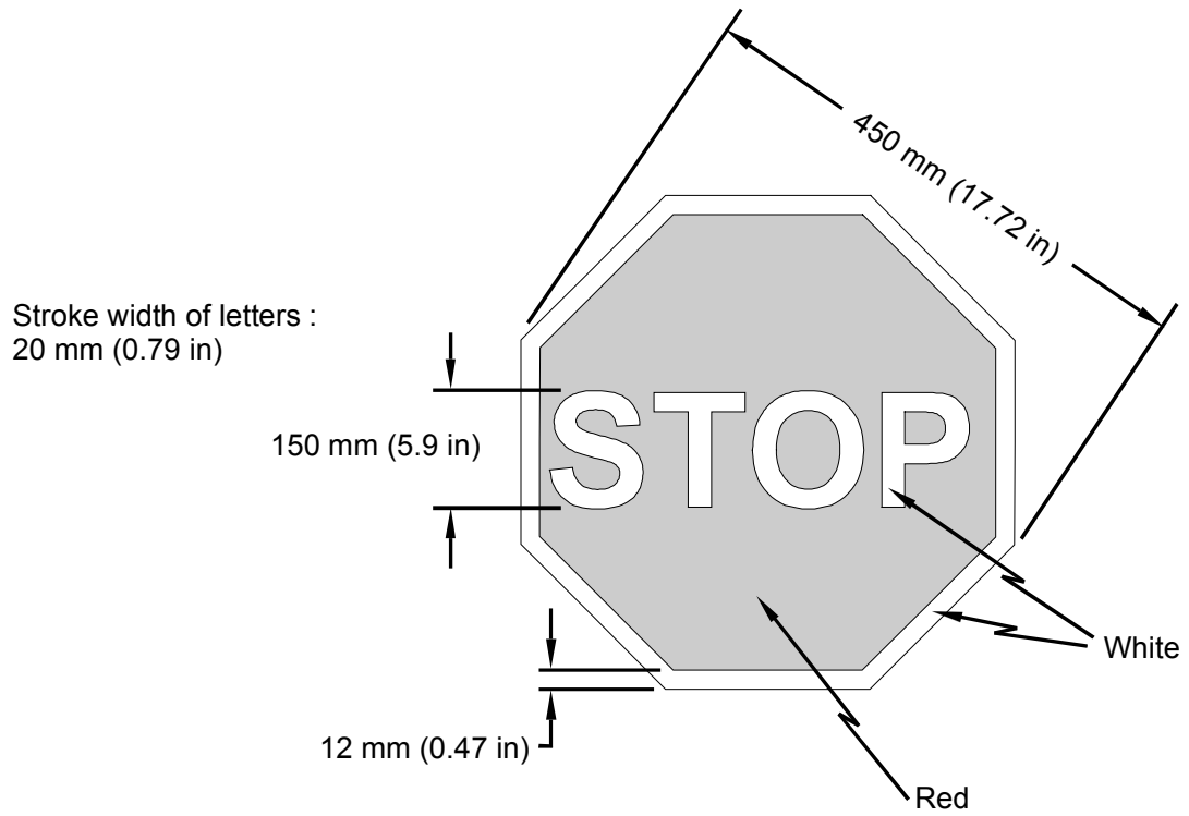
Figure 1: Characteristics of Stop Signal Device
