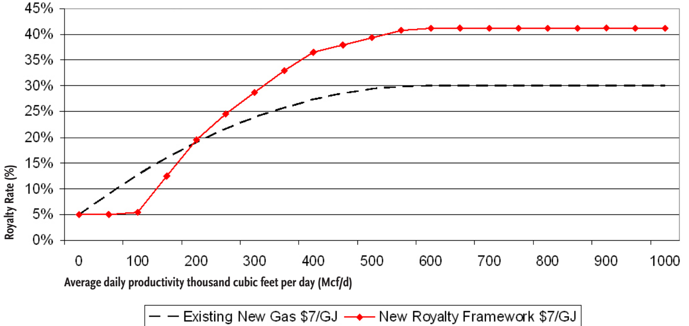
Natural Gas Royalty Curves — Well Productivity Comparison [based on gas price of $7 per gigajoule (GJ)]
