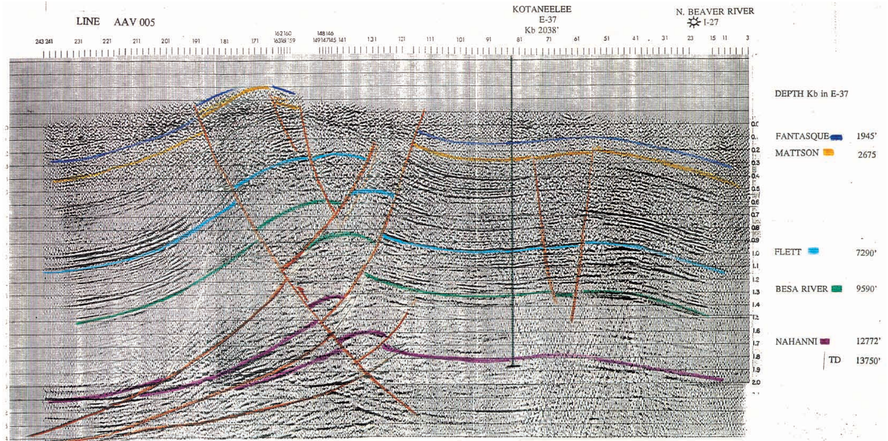
Figure 4 Seismic line AAV 005 Columbia Oil and Gas 1978. Interpretation NEB
