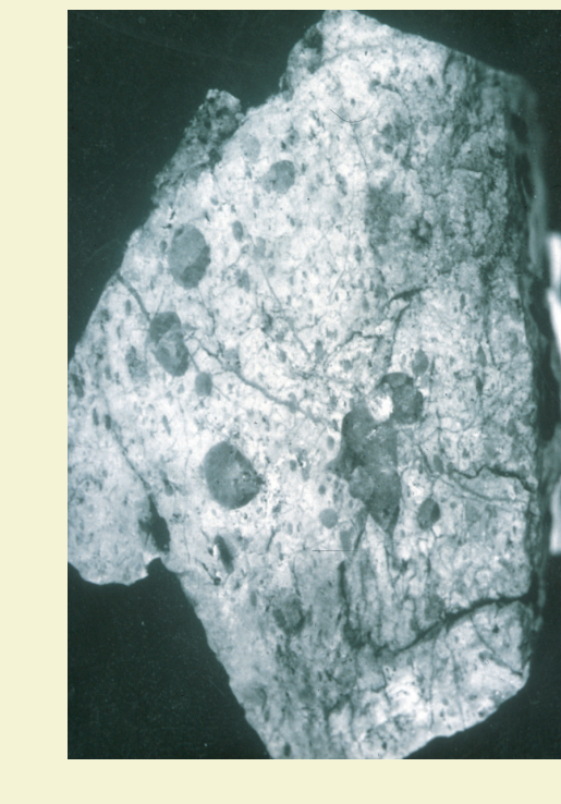
Amygdaloidal meta-rhyolite in hanging wall
