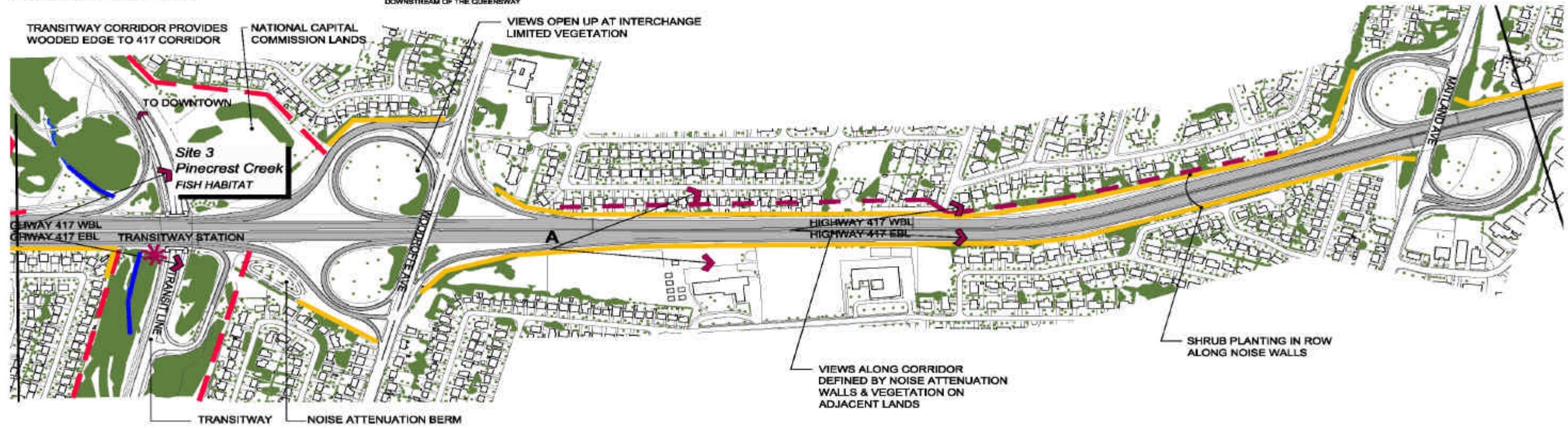
VIEW 'A' - EASTERLY FROM WOODROFFE AVENUE
