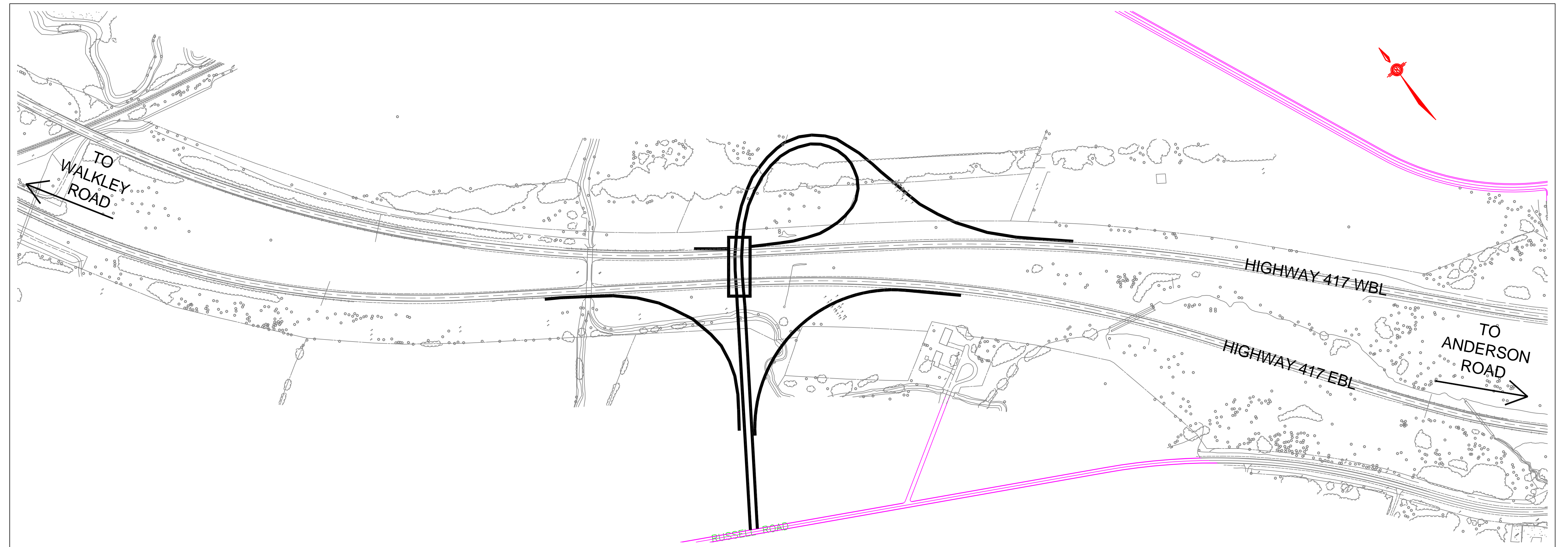
SKETCH A: "TRUMPET" INTERCHANGE CONFIGURATION
