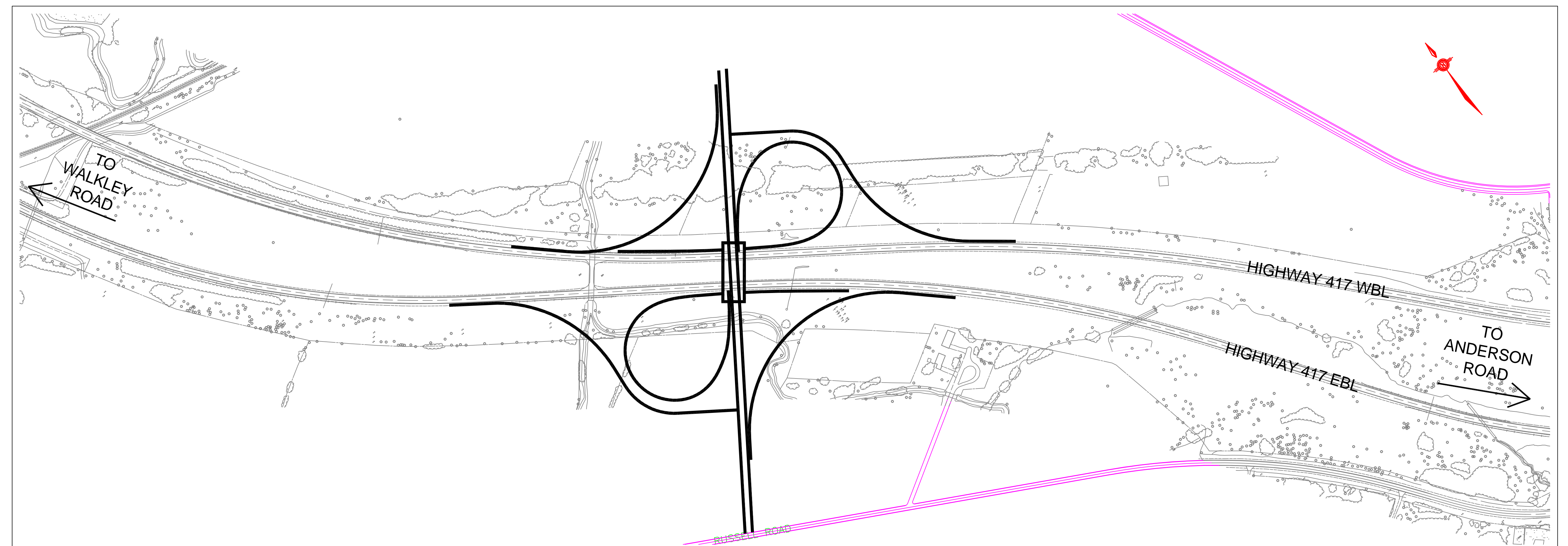
SKETCH B: "PARCLO A-4" INTERCHANGE CONFIGURATION
