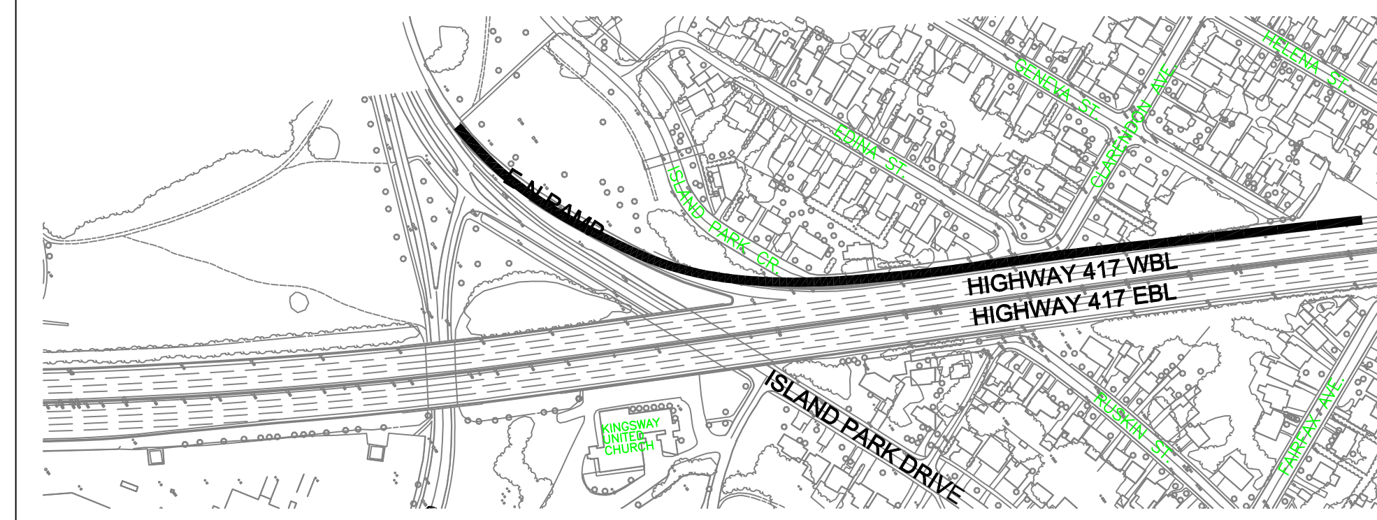
SKETCH 19-1: ADD DECELERATION LANE FOR ISLAND PARK WB OFF-RAMP
