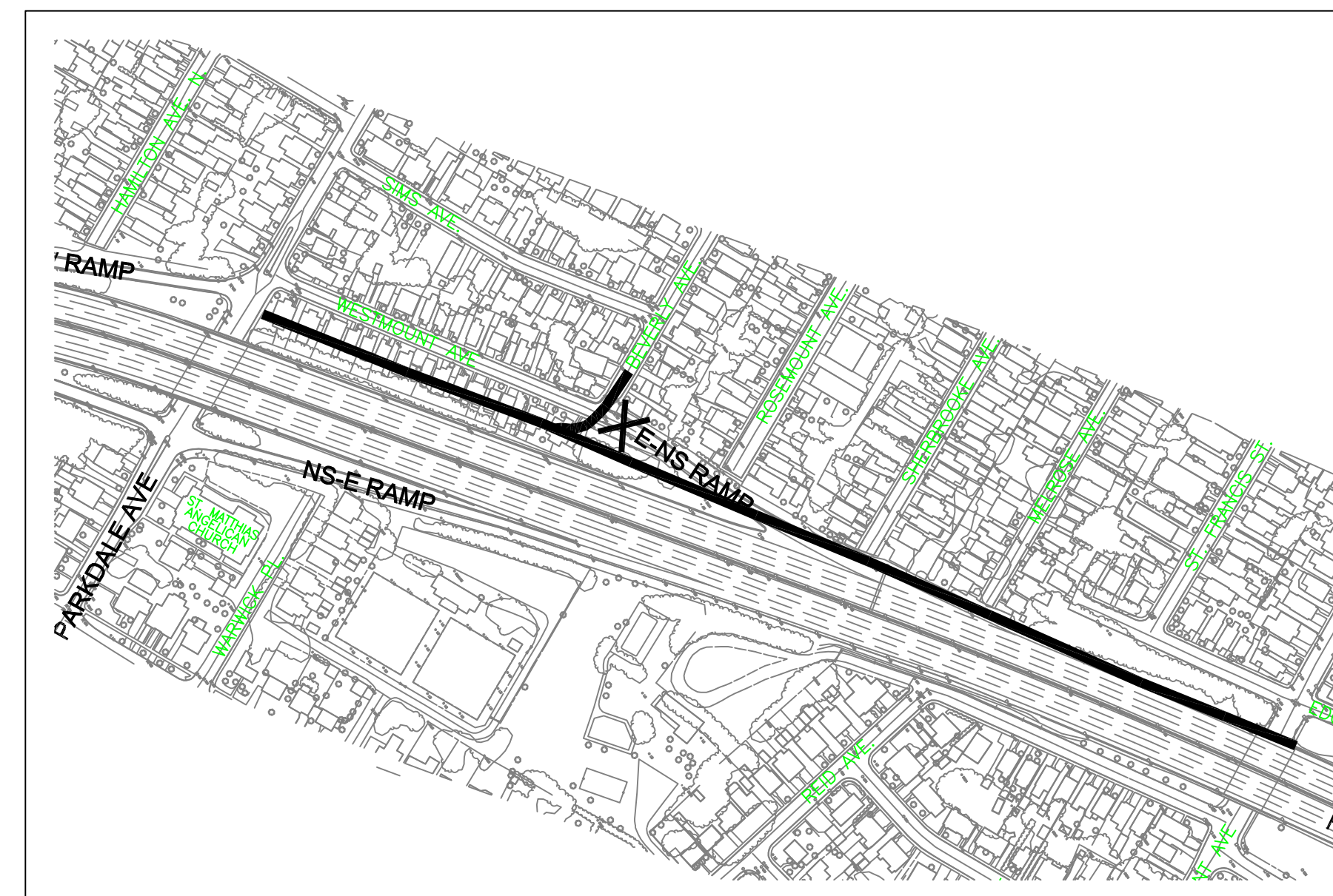
SKETCH 21: REALIGN WB OFF-RAMP TO THE SOUTH
