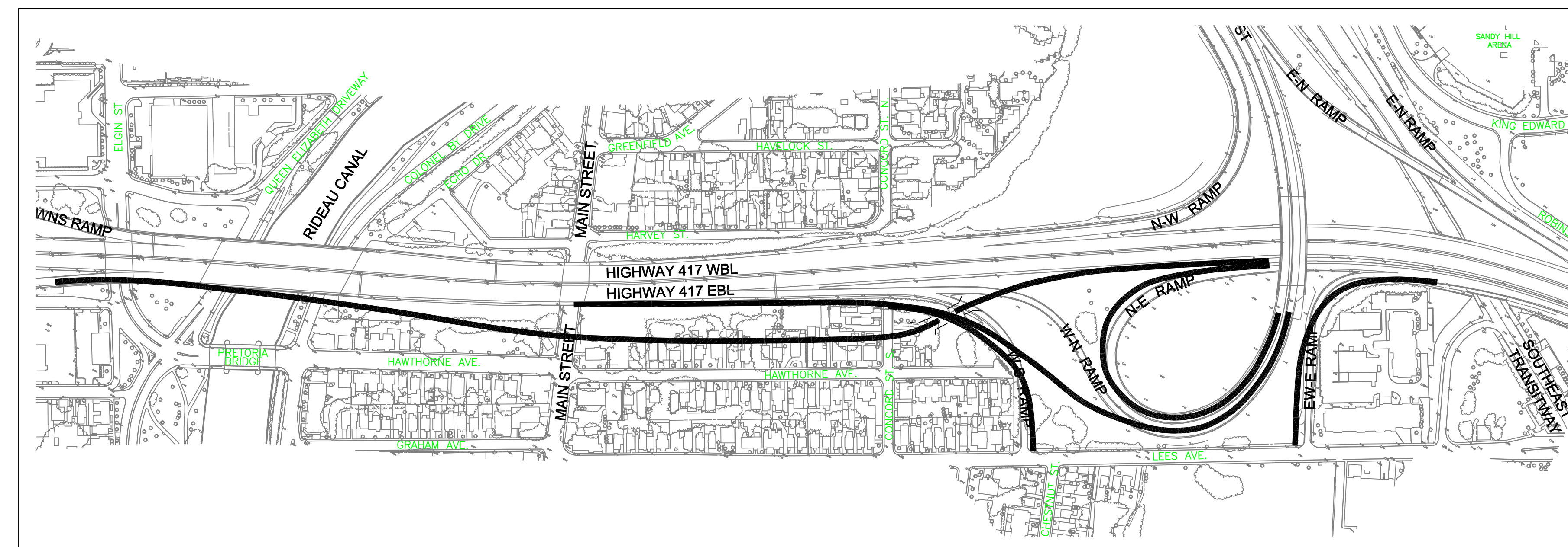
SKETCH 28: IMPROVE EB METCALFE ON-RAMP CAPACITY BY ELIMINATING WEAVE WITH EB OFF-RAMP TO NICHOLAS/LEES
