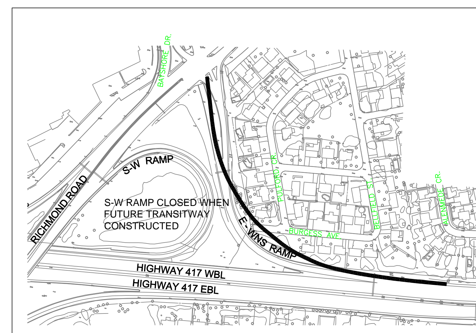
SKETCH 4: REALIGN OFF-RAMP TO IMPROVE CURVATURE AND OPERATIONS WHILE MAINTAINING CURRENT INTERSECTION AT RICHMOND ROAD
