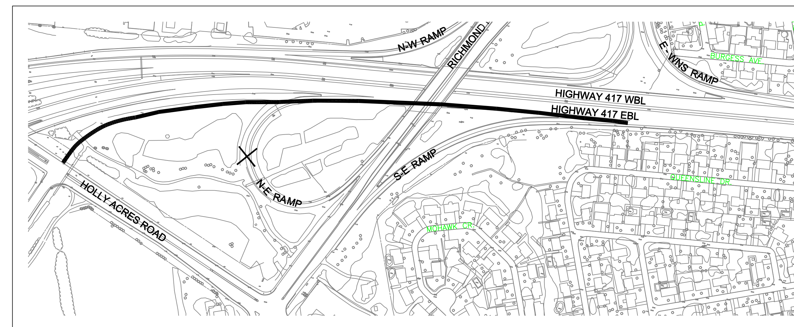
SKETCH 5: CLOSE RICHMOND ROAD SOUTHBOUND TO QUEENSWAY EB LOOP RAMP AND RELOCATE TO HOLLY ACRES ROAD
