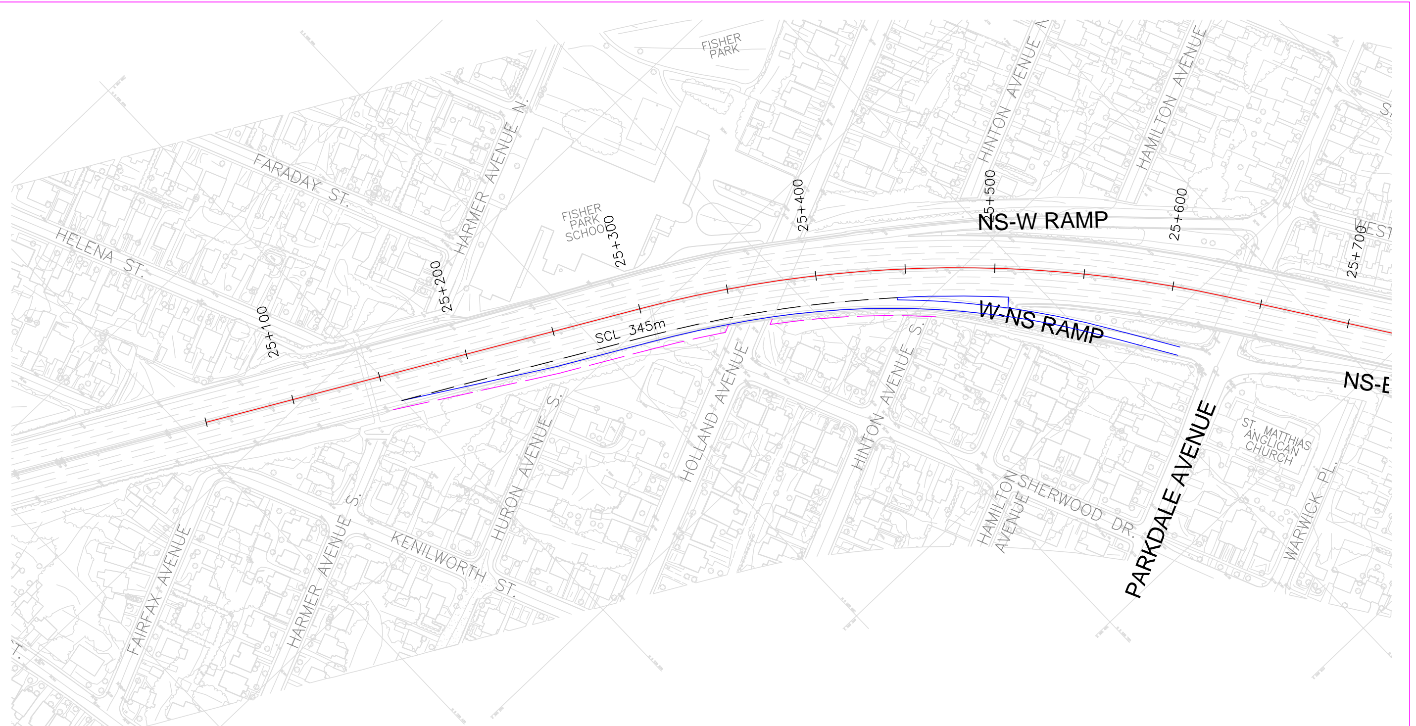
ALTERNATIVE 2 INCREASE LENGTH OF DECELERATION LANE FOR EB OFF-RAMP
