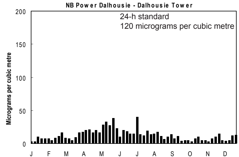
Daily TSP for 2006
