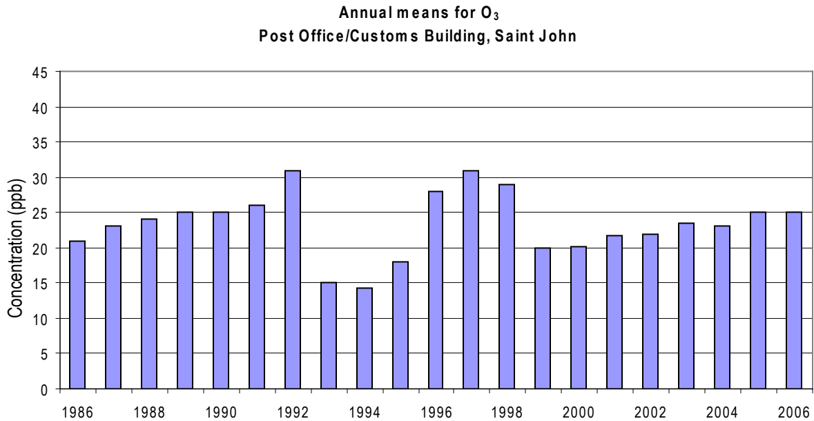
Figure 26. Annual mean ozone at Post Office/Customs Building, 1986-2006.
