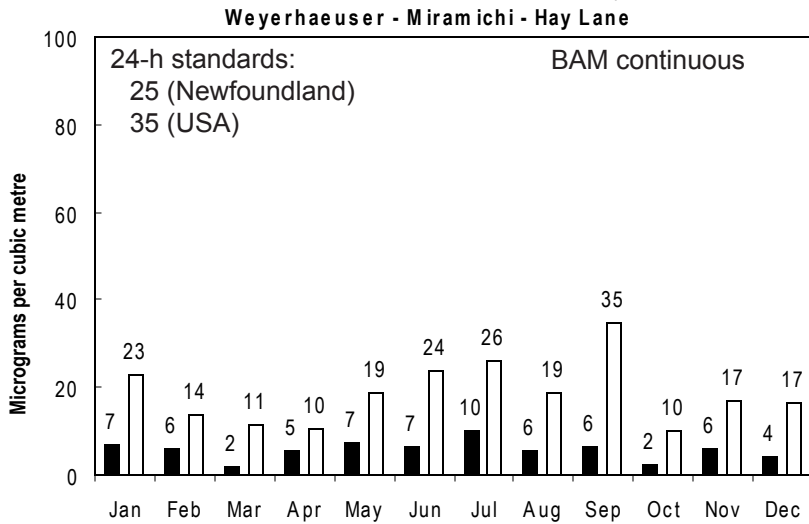
Monthly Average and Maximum 24-hour Values of PM 2.5 for 2006
