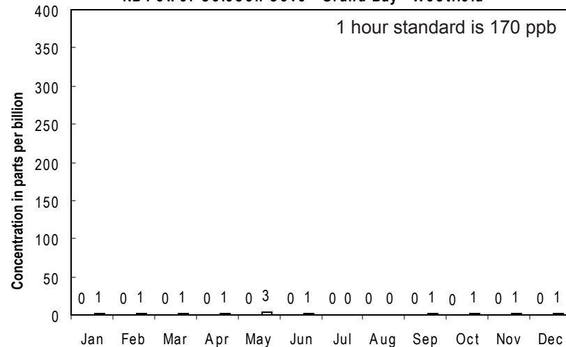
NB Power Coleson Cove - Grand Bay - Westfield
