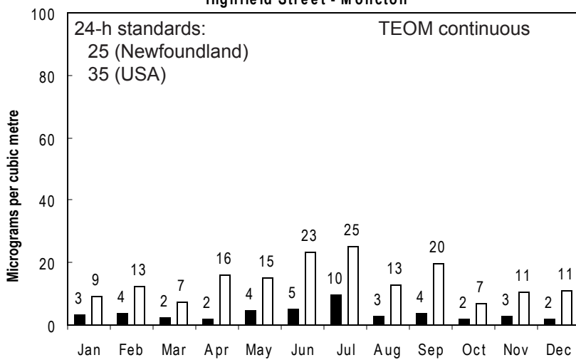
Monthly Average and Maximum 24-hour Values of PM 2.5 for 2006 Highfield Street - Moncton
