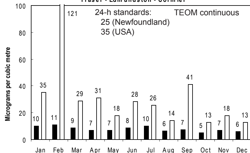
Monthly Average and Maximum 24-hour Values of PM 2.5 for 2006 Fraser - Edmundston - Cormier
