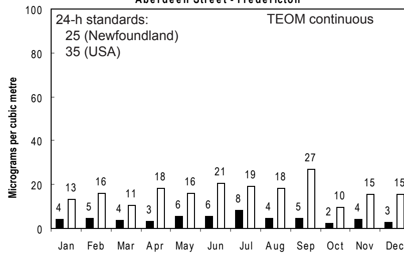
Monthly Average and Maximum 24-hour Values of PM 2.5 for 2006 Aberdeen Street - Fredericton
