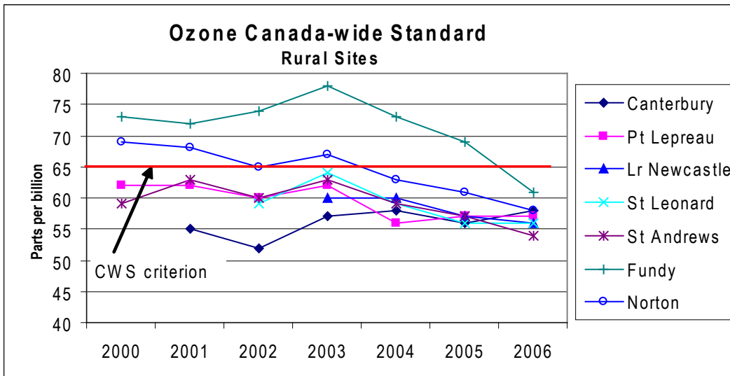
Figure 11. Canada-wide Standard results for ozone at rural sites, 2000-2006.
