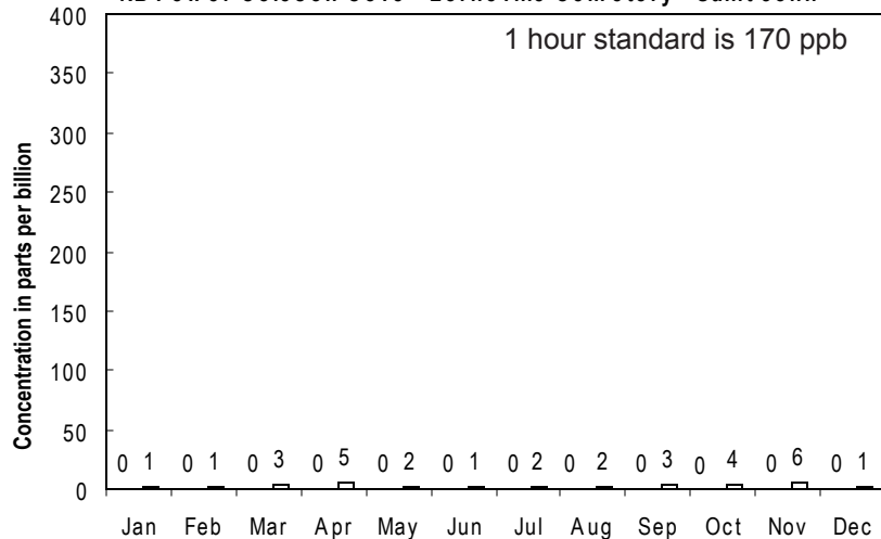
NB Power Coleson Cove - Lorneville Cemetery - Saint John
