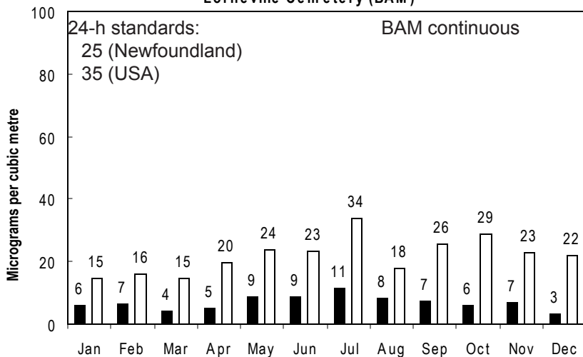
Monthly Average and Maximum 24-hour Values of PM 2.5 for 2006 Lorneville Cemetery (BAM)
