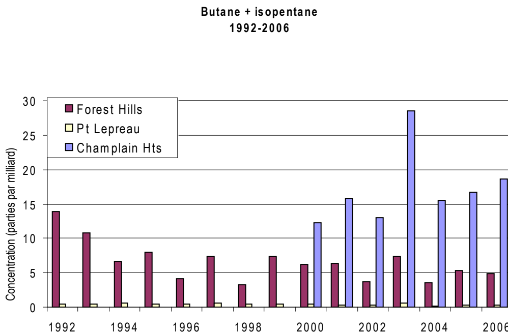
Figure 30. Annual average concentration of butane plus isopentane at provincial VOC monitoring sites, 1992-2006.
