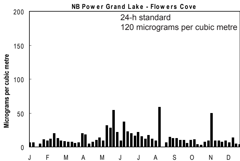
Daily TSP for 2006
