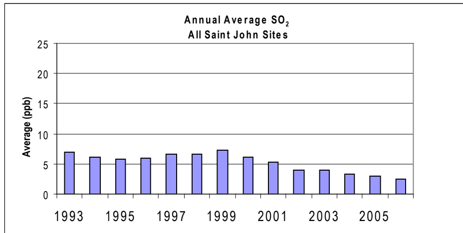
Figure 24. Trend in sulphur dioxide in Saint John, annual network average, 1993-2006.
