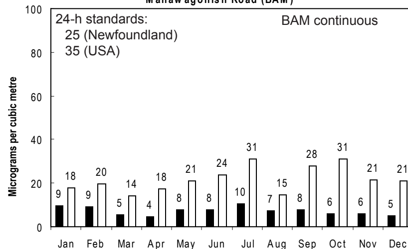
Monthly Average and Maximum 24-hour Values of PM 2.5 for 2006 Manawagonish Road (BAM)
