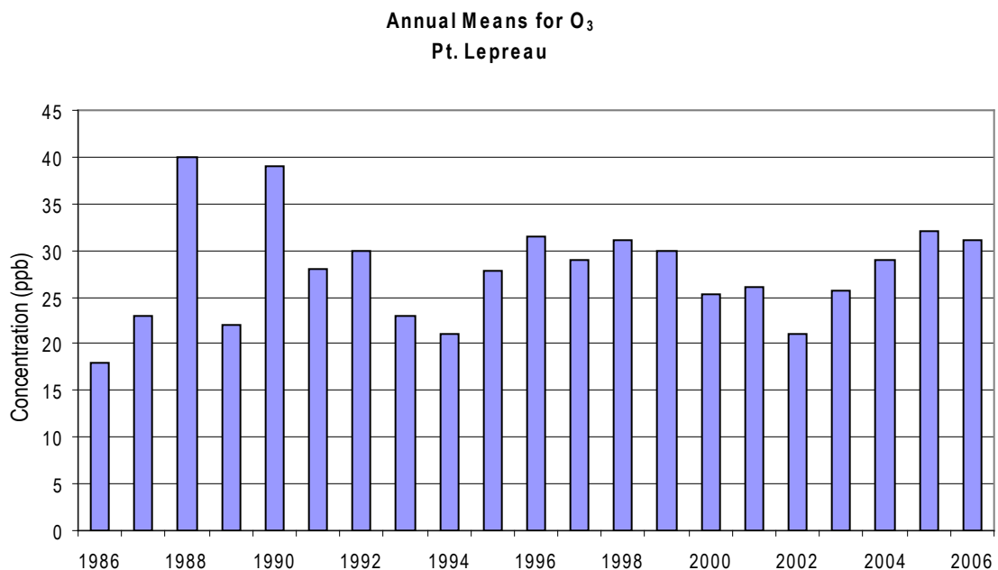
Figure 27. Annual mean ozone at Point Lepreau, 1986-2006.
