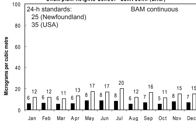
Monthly Average and Maximum 24-hour Values of PM 2.5 for 2006 Champlain Heights School - Saint John (BAM)
