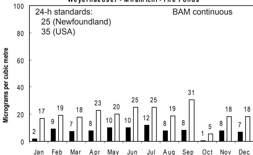
Monthly Average and Maximum 24-hour Values of PM 2.5 for 2006 Weyerhaeuser - Miramichi - Fire Ponds
