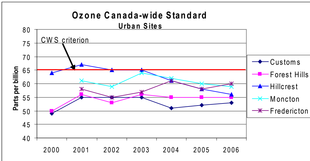
Figure 10. Canada-wide Standard results for ozone at urban sites, 2000-2006.
