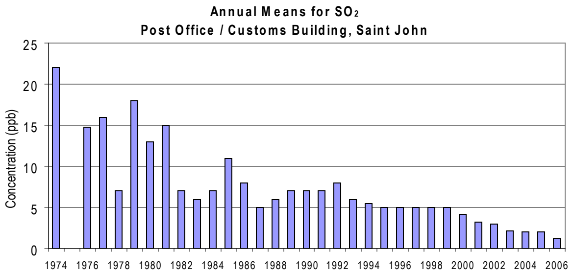
Figure 22. Annual mean sulphur dioxide at Post Office/Customs Building, Saint John, 1974-2006.
