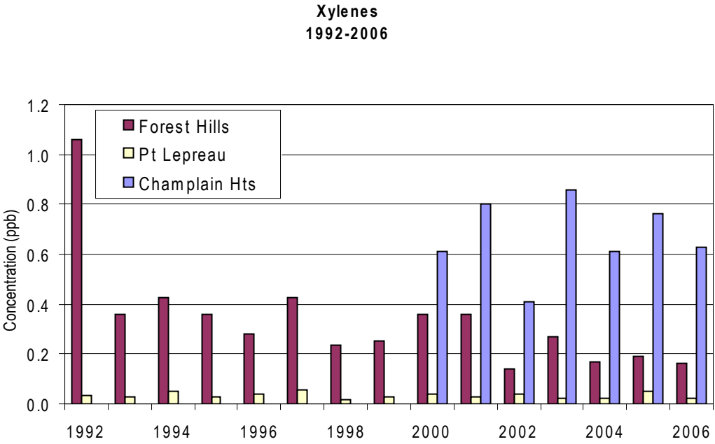
Figure 33. Annual average concentration of xylenes at provincial VOC monitoring sites, 1992-2006.
