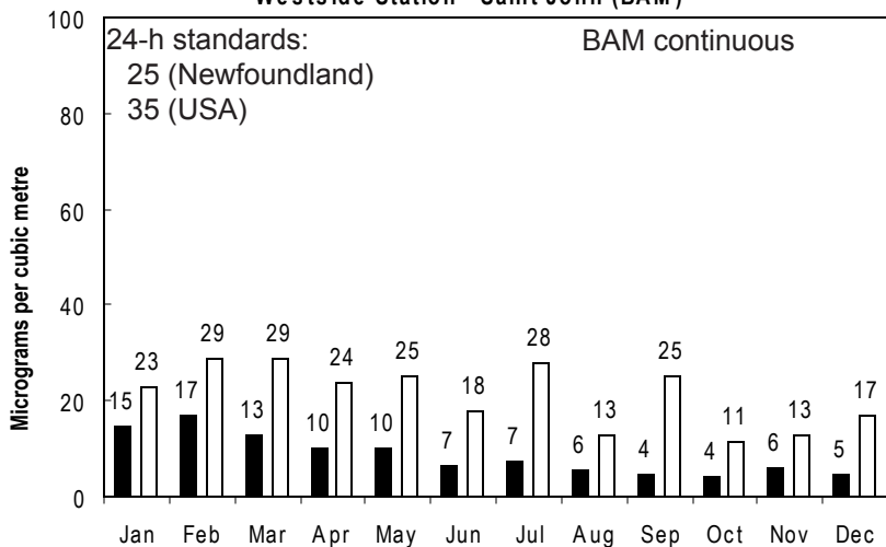
Monthly Average and Maximum 24-hour Values of PM 2.5 for 2006 Westside Station - Saint John (BAM)
