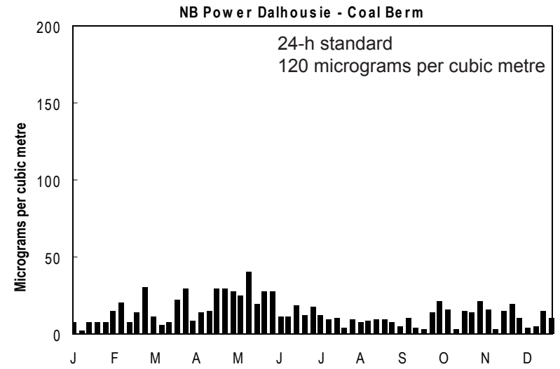
Daily TSP for 2006
