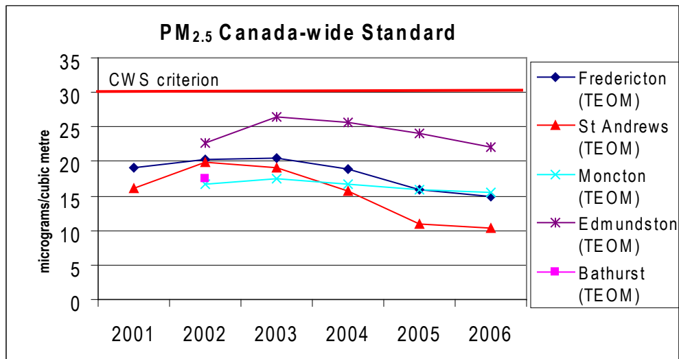
Figure 12. Canada-wide Standard results for PM 2.5 , 2001-2006.
