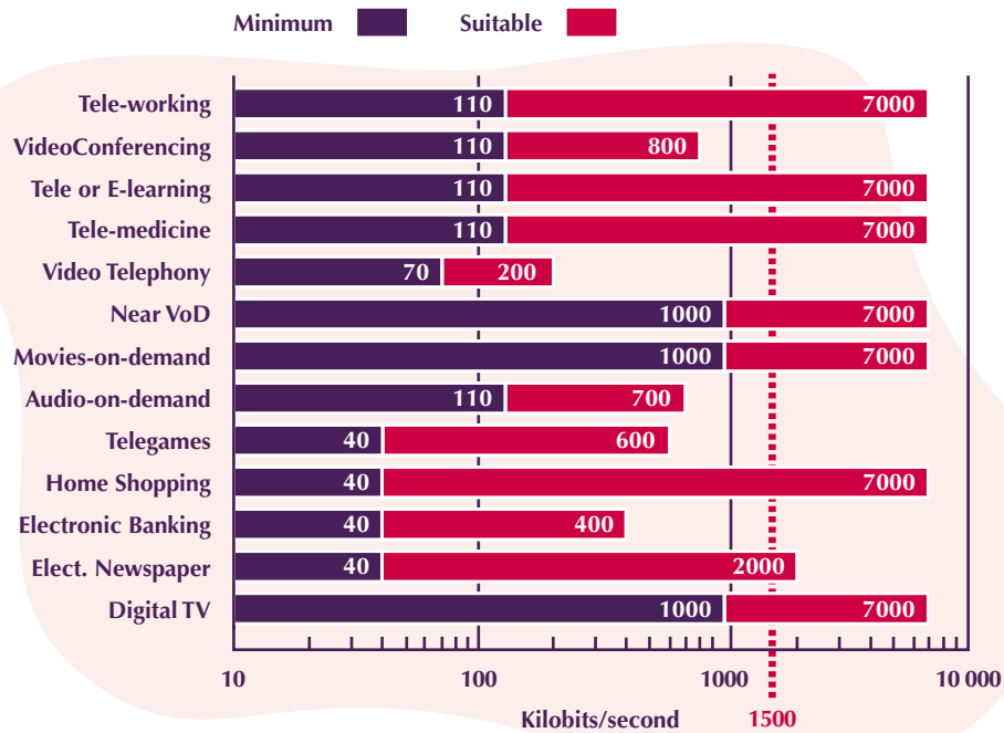
FIGURE 2 Bandwidth Requirements for Selected Applications Minimum and suitable speeds required by application
