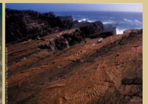
Mistaken Point
