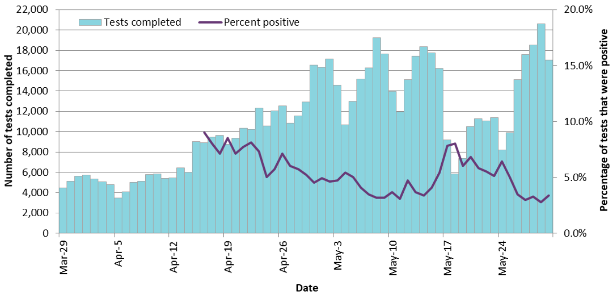
Figure 3. Number of COVID-19 tests completed 1 and percent positivity: Ontario, March 29, 2020 to May 30, 2020
