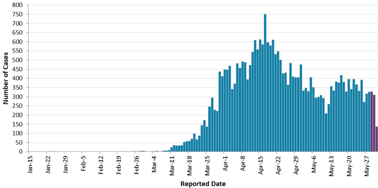
Figure 1. Confirmed cases (n=28,263) of COVID-19 by reported date: Ontario, January 15, 2020 to May 31, 2020 1
