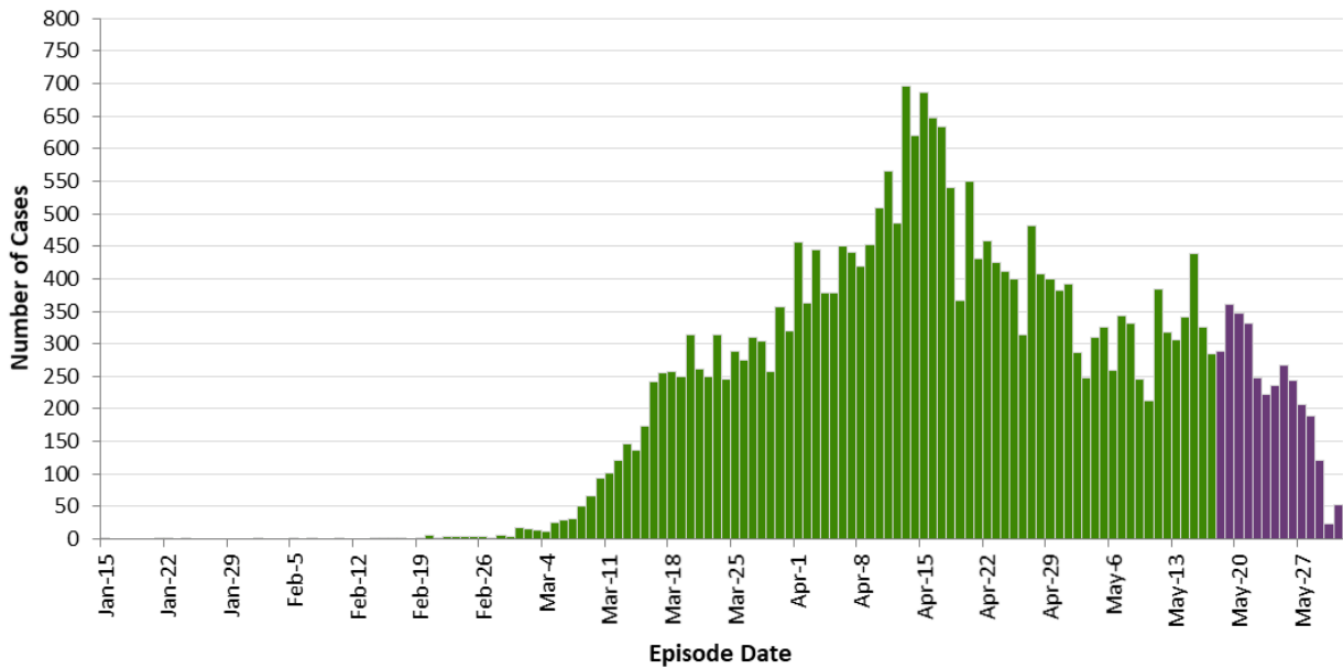
Figure 2. Confirmed cases (n=28,257 1 ) of COVID-19 by an approximation of symptom onset date 2 : Ontario, January 15, 2020 to May 31, 2020 3
