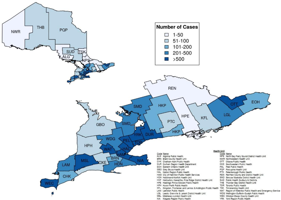
Figure 5. Confirmed cases (n=28,263) of COVID-19 by public health unit: Ontario, January 15, 2020 to May 31, 2020
