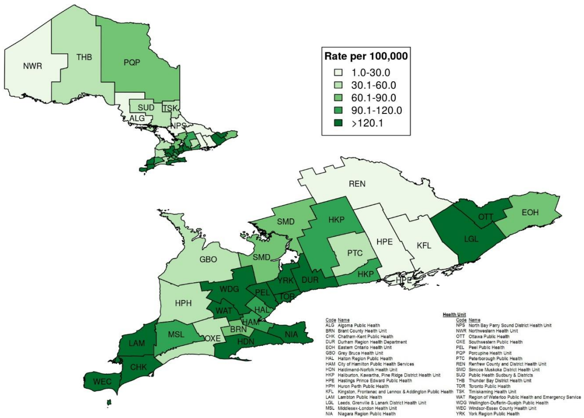
Figure 6. Rate of confirmed cases of COVID-19 by public health unit: Ontario, January 15, 2020 to May 31, 2020
