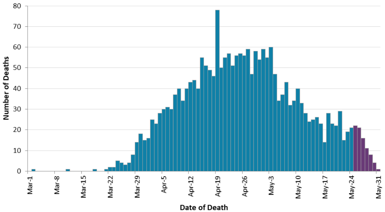
Figure 4. Confirmed deaths (n=2,273 1 ) among COVID-19 cases by date of death: Ontario, March 1, 2020 to May 31, 2020 2
