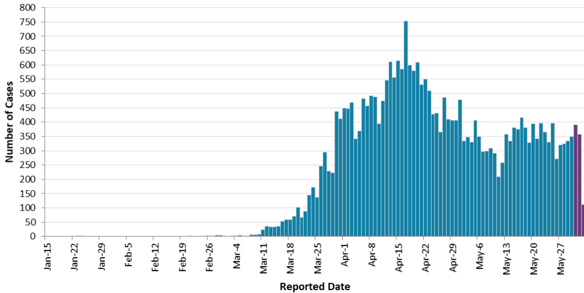
Figure 1. Confirmed cases (n=29,046 1 ) of COVID-19 by reported date: Ontario, January 15, 2020 to June 2, 2020 1
