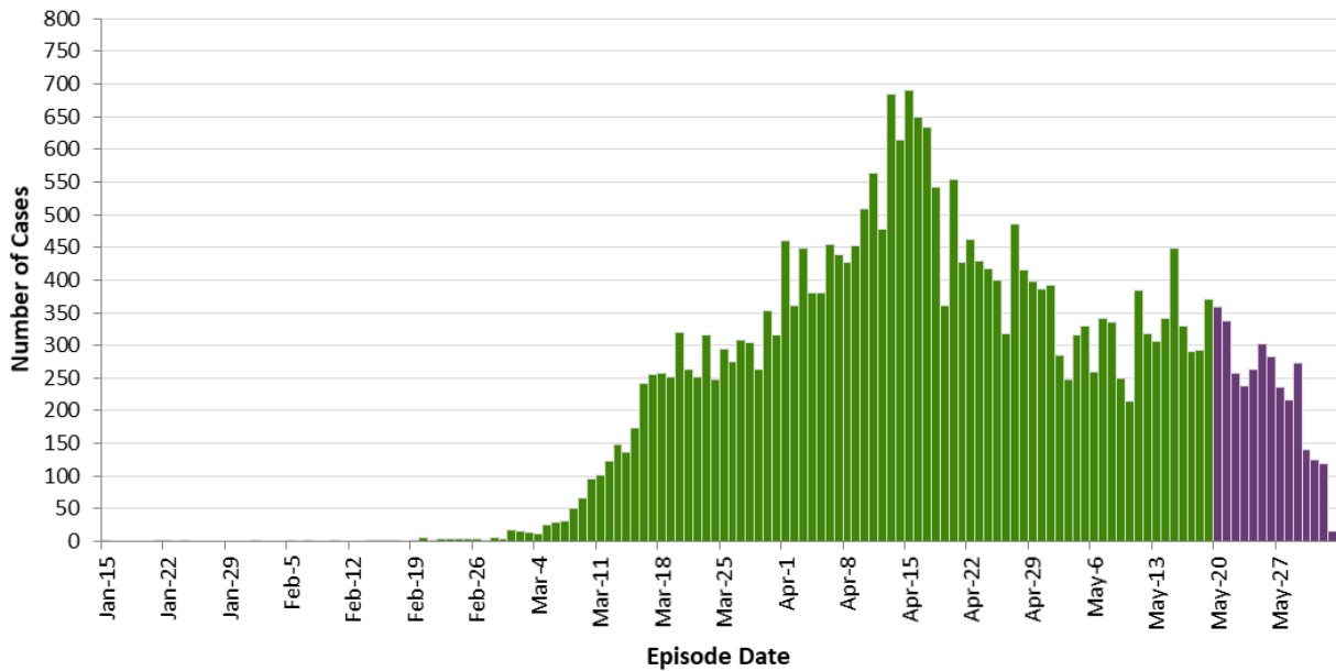
Figure 2. Confirmed cases (n=29,041 1 ) of COVID-19 by an approximation of symptom onset date 2 : Ontario, January 15, 2020 to June 2, 2020 3
