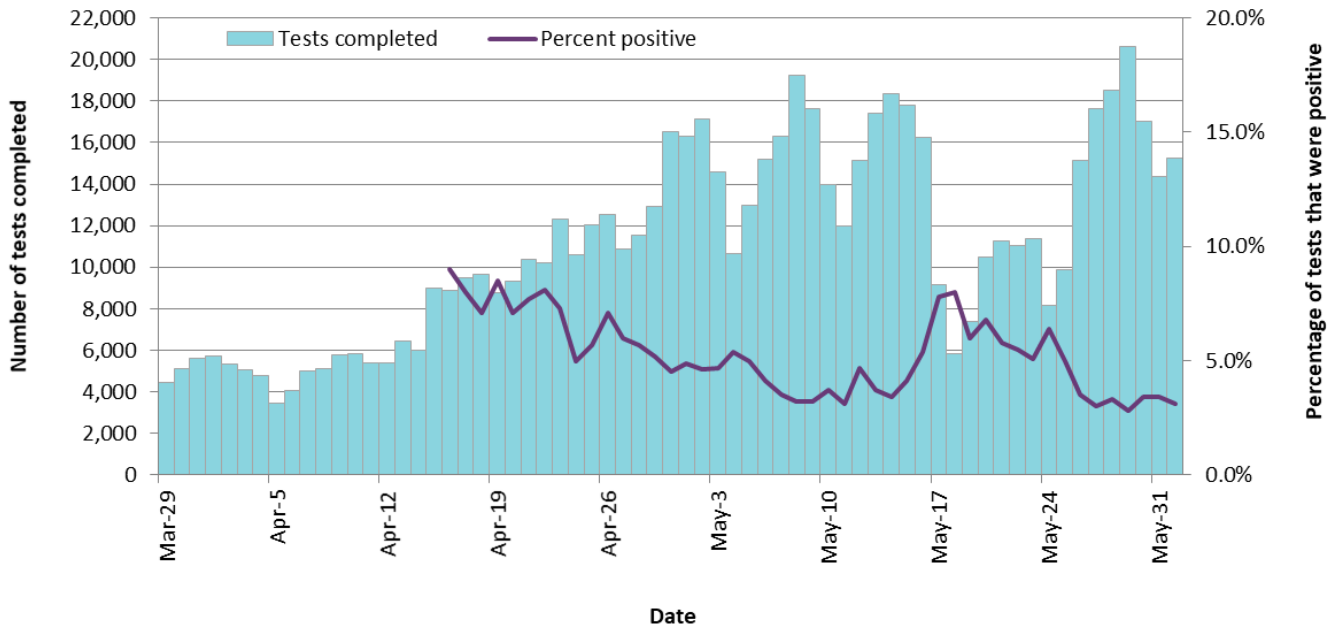
Figure 3. Number of COVID-19 tests completed 1 and percent positivity: Ontario, March 29, 2020 to June 1, 2020
