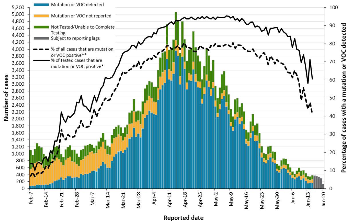
Figure 5. Number of confirmed COVID-19 cases and percent positive for mutations or VOCs: Ontario, February 7, 2021 to June 20, 2021
