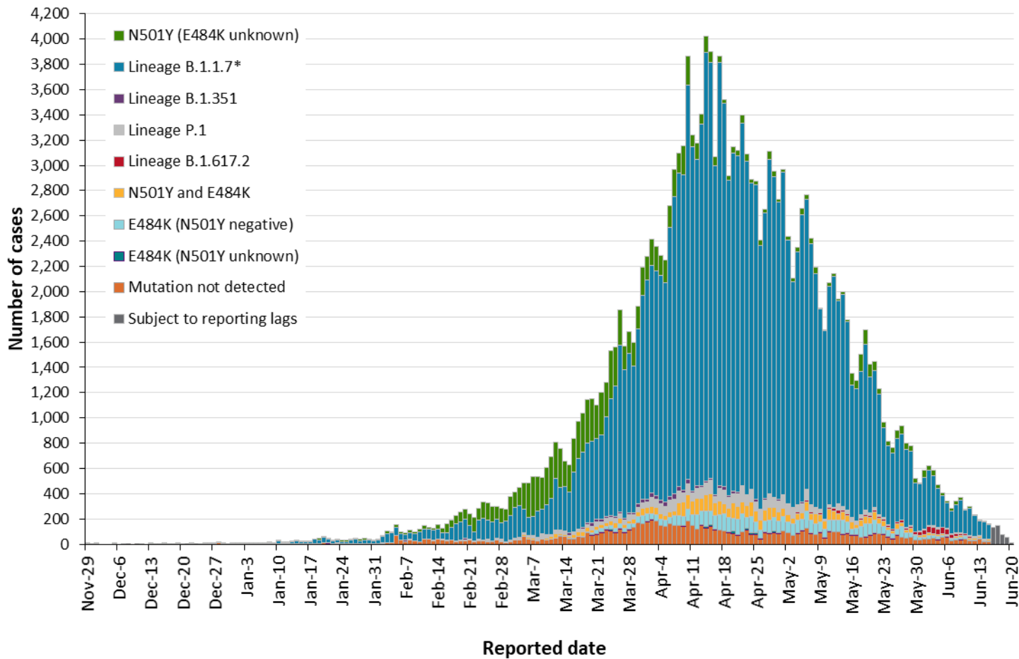
Figure 6. Confirmed COVID-19 cases with a mutation or VOC detected by public health unit reported date: Ontario, November 29, 2020 to June 20, 2021
