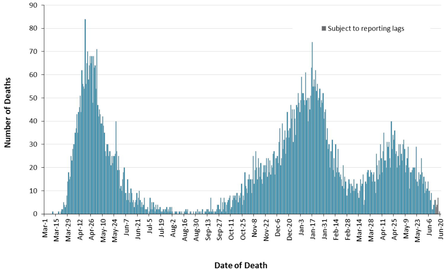
Figure 4. Confirmed deaths among COVID-19 cases by date of death: Ontario, March 1, 2020 to June 20, 2021
