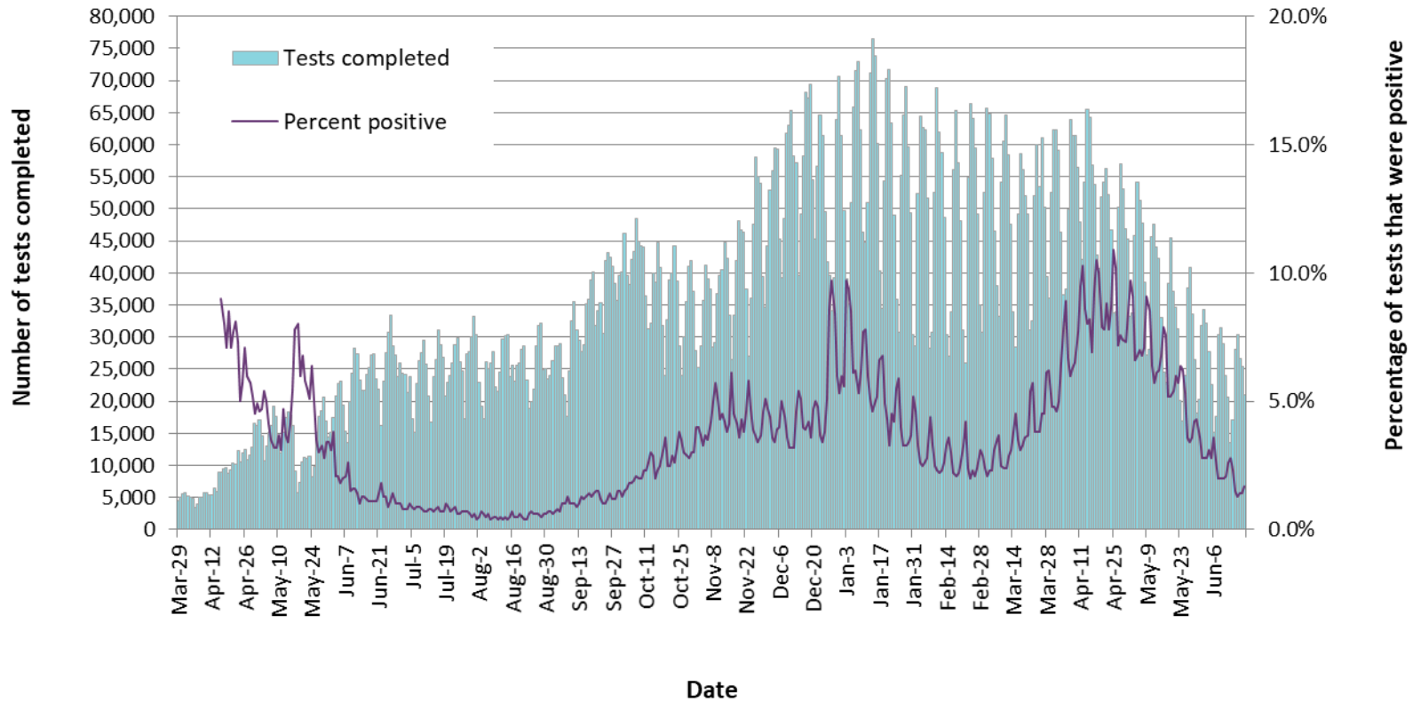
Figure 3. Number of COVID-19 tests completed and percent positivity: Ontario, March 29, 2020 to June 19, 2021
