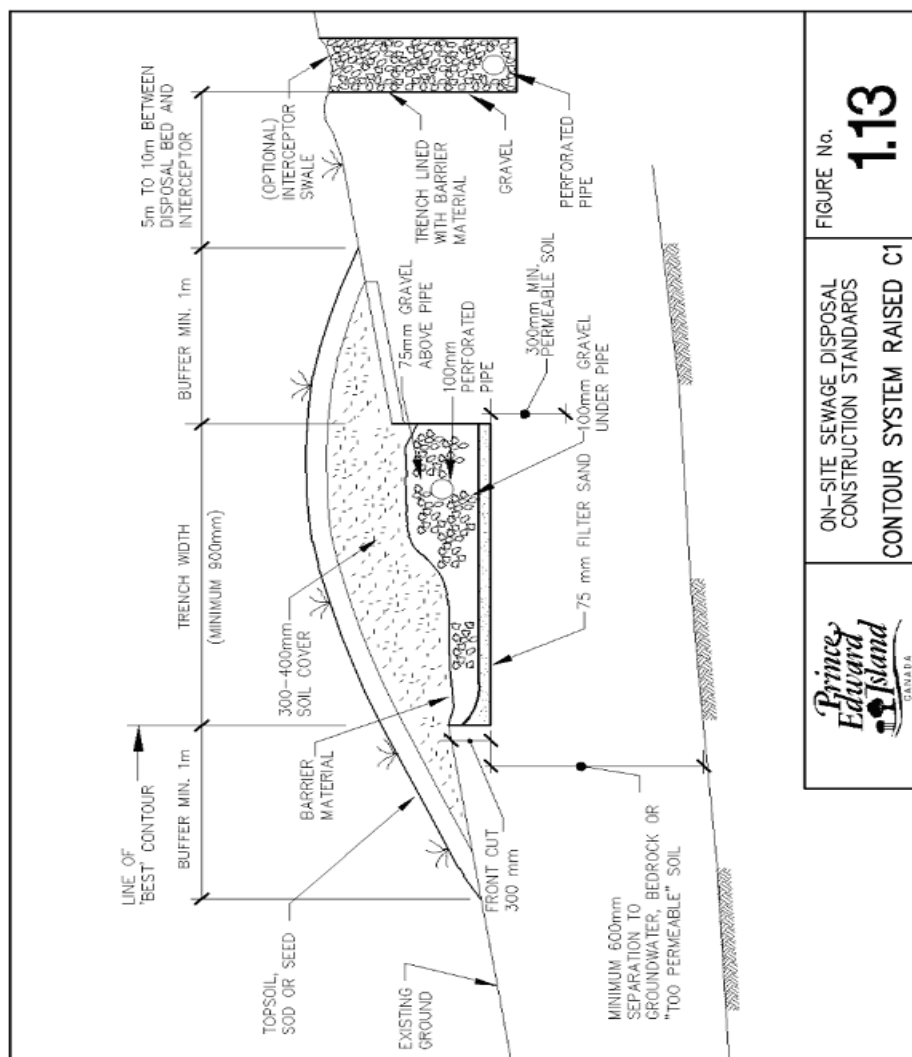
Figure 1.13 Contour System Raised C1
